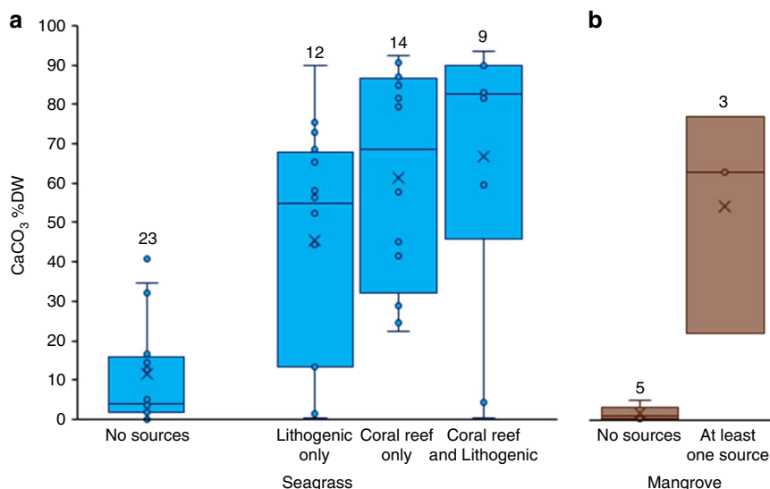
Fig. 4 Allochthonous sources and inorganic carbon in sediments. a %DW of carbonates (CaCO 3 ) in seagrass sediments depending on the presence of potential allochthonous sources (lithogenic and/or coral reefs). All data distributions for locations with allochthonous sources are significantly different to the distributions for locations without allochthonous sources (Mann–Whitney U -tests, all p < 0.001 ). b %DW CaCO 3 in mangrove sediments with and without allochthonous sources (coral reef and lithogenic source). Number on top of the box plots indicate the number of locations. The x represents the mean. Bars are the first and last quartile
