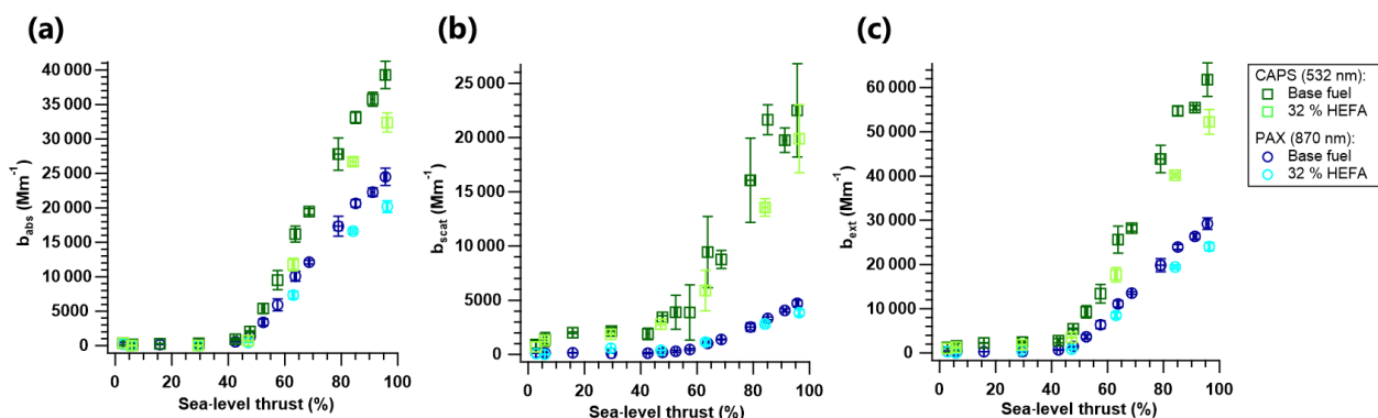
Figure 4. Thrust-dependent (a) absorption coefficient ( b_{\text{abs}} ), (b) scattering coefficient ( b_{\text{scat}} ) and (c) extinction coefficient ( b_{\text{ext}} ) measured at 532 nm (green squares) and 870 nm (blue circles). Note that dark colours represent measurements with base fuel (Jet A-1), and light colours represent measurements with the 32 % vol HEFA blend.
