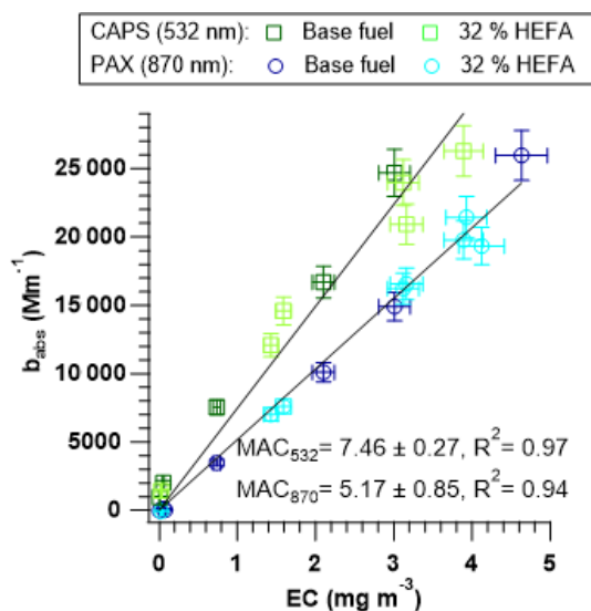
Figure 5. Scatter plot and linear regression lines between the absorption coefficient ( b_{\text{abs}} ) measured at 532 nm (green squares) and 870 nm (blue circles) and the elemental carbon (EC) mass concentration. Mass absorption cross section (MAC) values are retrieved from the slope of the linear fits. Note that dark colours represent measurements with base fuel (Jet A-1), and light colours represent measurements with the HEFA blend (32 % vol).
