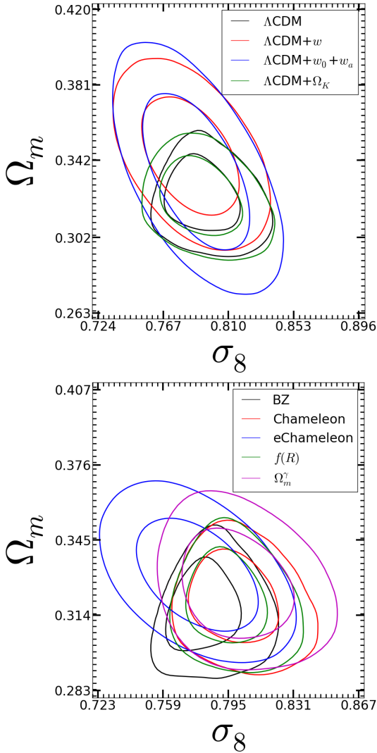
Figure 4. The figure shows the 1\sigma and 2\sigma regions for each of the models considered in this paper in \Omega_m - \sigma_8 plane. It shows that the posterior likelihood is consistent for each of the model in this parameter space. The top plots shows the models which are extension to \Lambda CDM and the bottom plot shows the modified gravity models.
