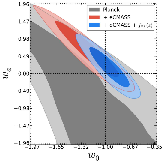
Figure 7. w_0w_a\text{CDM} : The two dimensional posterior likelihood of w_0 and w_a for time-dependent dark energy model. The grey contour is for Planck ( w_0 = -0.99 \pm 0.52 , w_a = -1.50 \pm 1.46 ), red contour is combined constraint from Planck and eCMASS ( w_0 = -1.23 \pm 0.26 , w_a = 0.63 \pm 0.49 ). The blue contour represents results from combining Planck with eCMASS and f\sigma_8(z) ( w_0 = -0.94 \pm 0.17 , w_a = 0.16 \pm 0.36 ).
