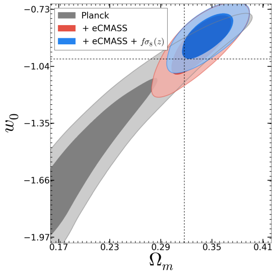
Figure 6. w\text{CDM} : The two dimensional posterior likelihood w and \Omega_m for w\text{CDM} . The grey contour is for Planck ( w_0 = -1.27 \pm 0.42 ), red contour is combined constraint from Planck and eCMASS ( w_0 = -0.92 \pm 0.10 ). The blue contour represents constraint from combining Planck with eCMASS and f\sigma_8(z) ( w_0 = -0.87 \pm 0.077 ).
