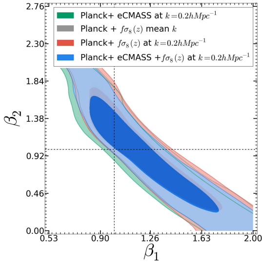
Figure 9. BZ: The two dimensional posterior likelihood of \beta_1 - \beta_2 for five parameter Scalar-tensor theory parametrized through the BZ form of (2). The green contour is the combined constraint from Planck and eCMASS ( \beta_1 = 1.18 \pm 0.29 , \beta_2 = 0.95 \pm 0.43 ). The grey contour is the combined constraint from Planck and f\sigma_8(z) with averaged over k ( \beta_1 = 1.24 \pm 0.3 , \beta_2 = 0.96 \pm 0.45 ), red contour is the combined constraint from Planck and f\sigma_8(z) at effective k = 0.2h \text{ Mpc}^{-1} ( \beta_1 = 1.24 \pm 0.3 , \beta_2 = 0.95 \pm 0.45 ). The blue contour represents results from the combination of Planck, f\sigma_8(z) and eCMASS ( \beta_1 = 1.23 \pm 0.29 , \beta_2 = 0.93 \pm 0.44 ).
