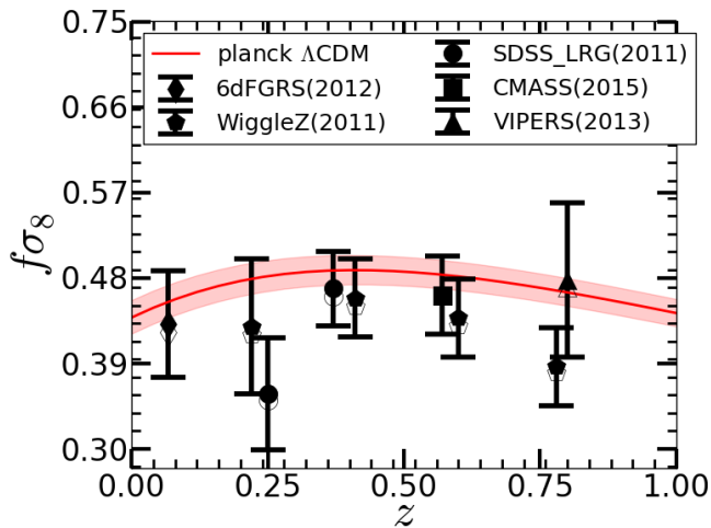
Figure 1. The measured f\sigma_8 from different surveys covering redshift range 0.06 < z < 0.8 . The empty markers represent the reported measurement of f\sigma_8 and the filled markers are for the corrected values for Planck Cosmology. The red band shows the Planck \Lambda CDM 1\sigma prediction.
