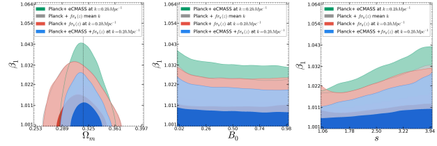
Figure 10. Chameleon Theory: The two dimensional posterior likelihood for Chameleon gravity. The green contour is the combined constraint from Planck and eCMASS ( \beta_1 < 1.013 ). The grey contour is the combined constraint from Planck and f\sigma_8(z) with averaged over k ( \beta_1 < 1.010 ), the red contour is the combined constraint from Planck and f\sigma_8(z) at effective k = 0.2h \text{ Mpc}^{-1} ( \beta_1 < 1.010 ). The blue contour represents results from the combination of Planck, eCMASS and f\sigma_8(z) ( \beta_1 < 1.008 ).
