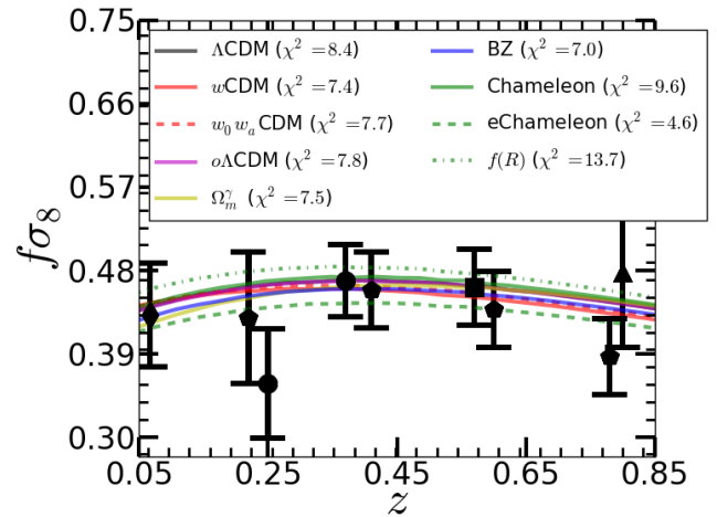
Figure 3. The black points show the corrected f\sigma_8 used in our analysis, along with the errorbar. Lines of different colors show the best fit for the various models used in our analysis. The best fit and \chi^2 are for the case of Planck + f\sigma_8 + eCMASS fits. Notice that the eChameleon model predicts the smallest growth rate by preferring lower values of the coupling constant ( \beta_1 ), even though the scalar amplitude of primordial power spectrum is high.
