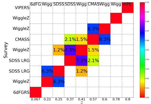
Figure 2. Correlation matrix between all the measurements used in our analysis. We have estimated the correlation as the fraction of overlap volume between two survey to the total volume of the two surveys combined.
