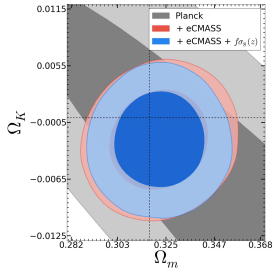
Figure 8. o\Lambda\text{CDM} : The two dimensional posterior likelihood of \Omega_k and \Omega_m for o\Lambda\text{CDM} . The grey contour is for Planck ( \Omega_k = -0.060 \pm 0.047 ), red contour is combined constraint from Planck and eCMASS ( \Omega_k = -0.0024 \pm 0.0034 ). The blue contour represents results from combining Planck with eCMASS and f\sigma_8(z) ( \Omega_k = -0.0024 \pm 0.0032 ).
