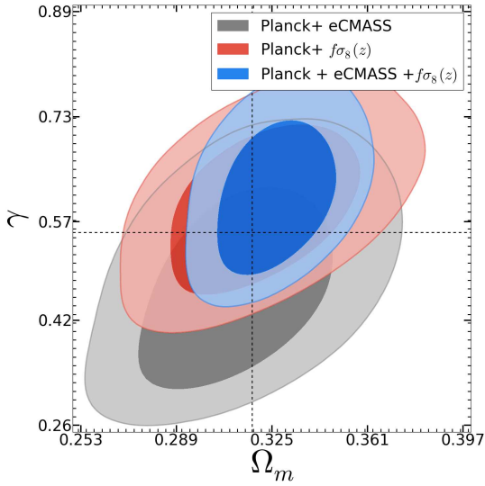
Figure 13. Growth index ( \gamma ): The two dimensional posterior likelihood of \gamma and \Omega_m for growth index parametrization. The grey contour is the combined constraint from Planck and eCMASS ( \gamma = 0.477 \pm 0.096 ). The red contour is the combined constraint from Planck and f\sigma_8(z) ( \gamma = 0.595 \pm 0.079 ). The blue contour represents results from the combination of Planck, f\sigma_8(z) and eCMASS ( \gamma = 0.612 \pm 0.072 )
