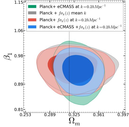
Figure 11. eChameleon Theory: The two dimensional posterior likelihood of \beta_1 and \Omega_m for extended Chameleon gravity. The green contour is the combined constraint from Planck and eCMASS ( \beta_1 = 0.932 \pm 0.04 ). The grey contour is the combined constraint from Planck and f\sigma_8(z) with averaged over k ( \beta_1 = 0.940 \pm 0.032 ), red contour is combined constraint from Planck and f\sigma_8(z) at effective k = 0.2h \text{ Mpc}^{-1} ( \beta_1 = 0.936 \pm 0.032 ). The blue contour represents results from the combination of Planck, f\sigma_8(z) and eCMASS ( \beta_1 = 0.932 \pm 0.031 ).
