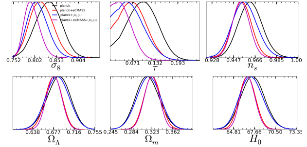
Figure 5. \Lambda CDM: We use GR as the model for gravity to determine the growth factor and fit for f\sigma_8(z) and eCMSS measurement with Planck likelihood. The black line shows the constraints from Planck 2013 alone. The red, blue and magenta lines are posterior obtained for the data set combinations \text{planck}+\text{eCMSS} , \text{planck}+f\sigma_8(z) and \text{planck}+\text{eCMSS}+f\sigma_8(z) respectively. The two most prominent effect are in optical depth \tau and scalar amplitude of primordial power spectrum A_s . Which is also reflected in the derived parameter \sigma_8 and mid redshift of re-ionization z_{re} .
