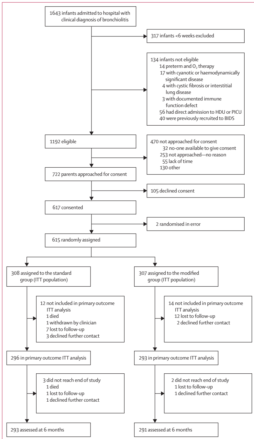
Figure 1: Study profile
