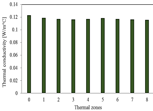
Fig. 7. Local measured thermal conductivity of the T1 sample for 10 W Heat flux, T_{coolant}=5^{\circ}C
