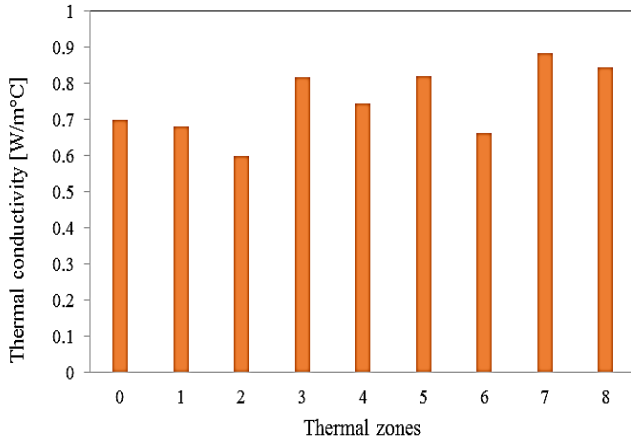
Fig. 6. Local measured thermal conductivity of the S3 sample for 10 W Heat flux, T_{coolant}=5^{\circ}C
