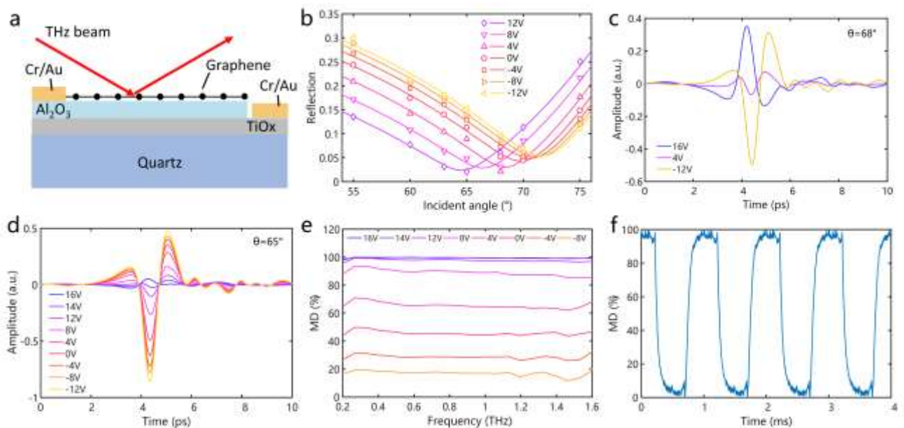
Figure 10. (a) Schematic of the graphene-quartz device. (b) Reflection as a function of incident angles Symbols are experimental data. Solid curves are theoretical calculations. (c) The time domain signals
