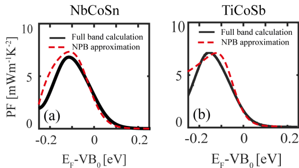
FIG. 14. Comparison of results from the non-parabolic band (NPB) approximation (red-dashed lines) and numerical full-band calculations (black-solid lines) using BoltzTraP, under the constant relaxation time approximation with \tau = 10^{-14} s, for (a) NbCoSn and (b) TiCoSb.
