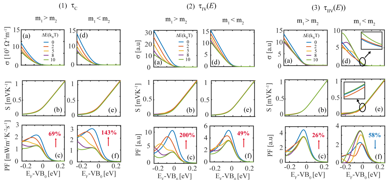
FIG. 2. Thermoelectric coefficients when aligning bands with different mass combinations under three scattering scenarios: Panel (1) for constant rate/time of scattering ( \tau_C ), panel (2) for intra-band scattering only ( \tau_{IV}(E) ) and panel (3) for inter- and intra-band scattering ( \tau_{IIV}(E) ). Each panel shows the coefficients: (a) electronic conductivity, (b) Seebeck coefficient, and (c) power factor when the mass of B1 is larger than that of B2, i.e. m_1 > m_2 ( m_1 = 1m_0, m_2 = 0.5m_0 ). Sub-figures (d-f) in each panel show the (d) electronic conductivity, (e) Seebeck coefficient, and (f) power factor when the mass of B1 is smaller than that of B2, i.e. m_1 < m_2 ( m_1 = 1m_0, m_2 = 2m_0 ).
