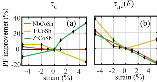
FIG. 12. Percentage improvement of the power factor (from peak to peak) under: (a) constant rate of scattering ( \tau_c ), and (b) inter- and intra-band\inter- and intra-valley scattering ( \tau_{IV}(E) ) versus strain percentage is applied for NbCoSn, TiCoSb and ZrCoSb. Positive strain indicates expansion while negative strain indicates compression.
