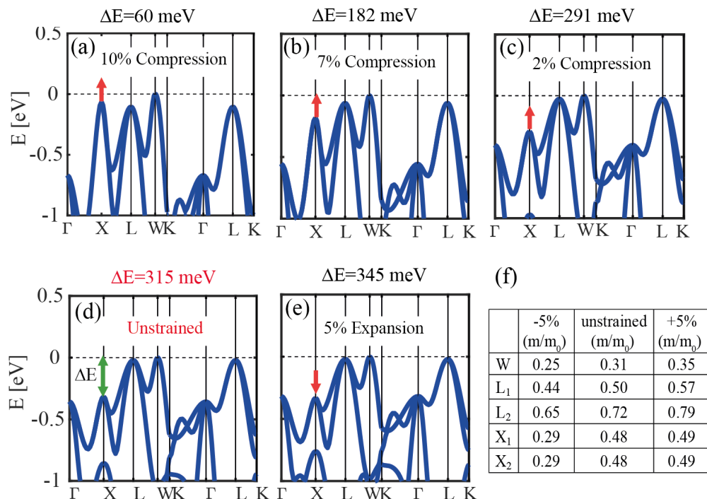
FIG. 6. (a)-(e) Application of strain in NbCoSn to align the X valley with the valence band edge. Strain values are as indicated in the figures, with (d) showing the unstrained bandstructure. (f) The calculated effective masses for the relevant bands at L, W and X valleys of NbCoSn using the parabolic band approximation for different strain levels [-5% (compressive), unstrained, and +5% (tensile)]. The energy separation \Delta E between the X valley and VB_0 are noted above the sub-figures.
