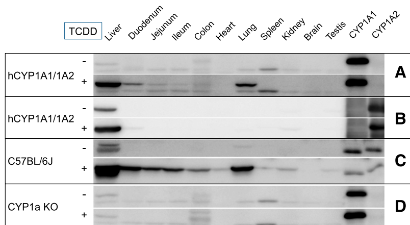
Fig. 2. Basal and TCDD-inducible expression of Cyp1a/CYP1A1 in tissues from WT, Cyp1a KO, and hCYP1A1/1A2 mice. Microsomes were prepared from vehicle (corn oil) and TCDD-treated hCYP1A1/1A2, Cyp1a KO, and WT mice from the tissues shown and immunoblotted for hCYP1A1 (A and D), human CYP1A2 (B), and mouse Cyp1a (C) as detailed in Materials and Methods . Standards: CYP1A1 (0.36 pmol/lane) and CYP1A2 (1 pmol/lane) expressed in bacterial membranes.
