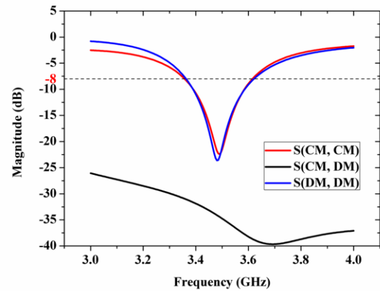
Fig. 9. Simulated S-parameters.
