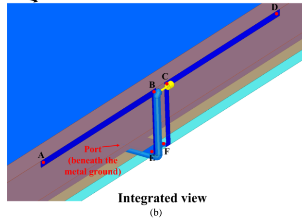
Fig. 7. A DM antenna on the side-edge of a smart phone. (a) Overall view. (b) Enlarged view.
