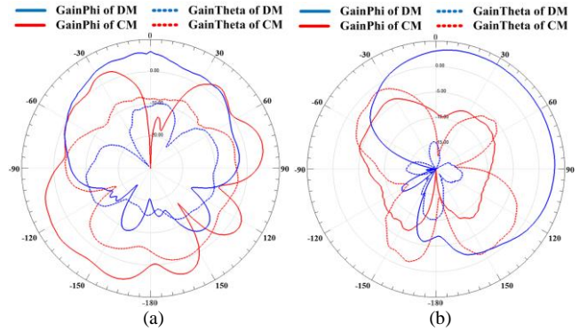
Fig. 23. Measured 2D patterns of Unit 3 at 3.5 GHz. (a) Plane XOY ( \phi = -180^\circ \sim 180^\circ ). (b) Plane XOZ ( \theta = -180^\circ \sim 180^\circ ).
