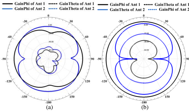
Fig. 6. 2D patterns of Ant 1 and Ant 2 at 3.5 GHz. (a) Plane XOY. (b) Plane YOZ.
