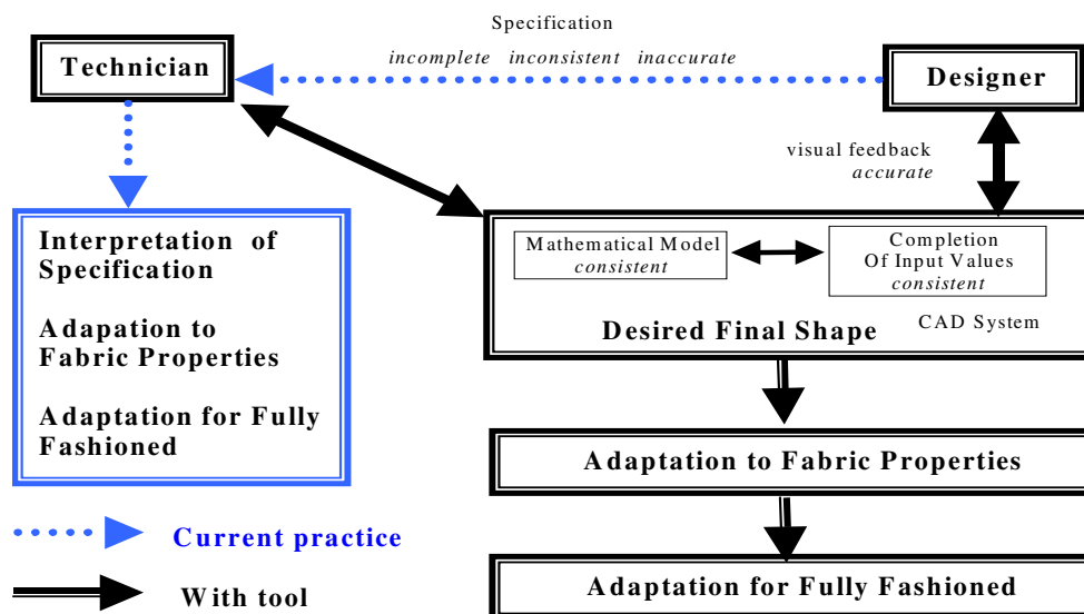
Figure 4. Communication Through an Automatic Shape Design System
