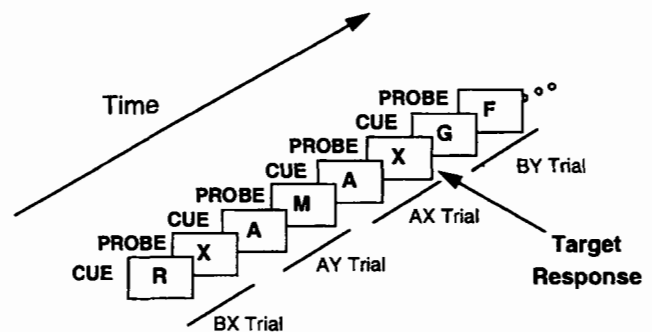
Figure 2. Schematic of AX-Continuous Performance Test paradigm. Single letters are visually displayed as a series of cue–probe pairs. A target is defined as the occurrence of an X probe immediately following an A cue. There are three types of nontarget trials: BX, AY, and BY (where B refers to any non-A cue, and Y refers to any non-X probe).
