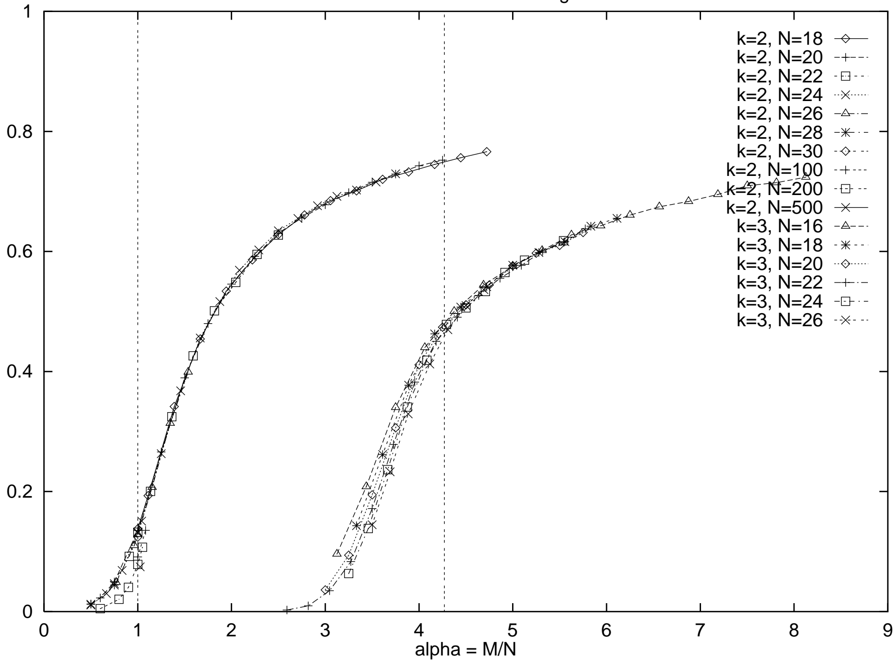
Backbone fractions for k=2 and k=3 ground states
