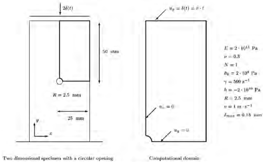
Figure 7. Rectangular specimen with one centred imperfection.
