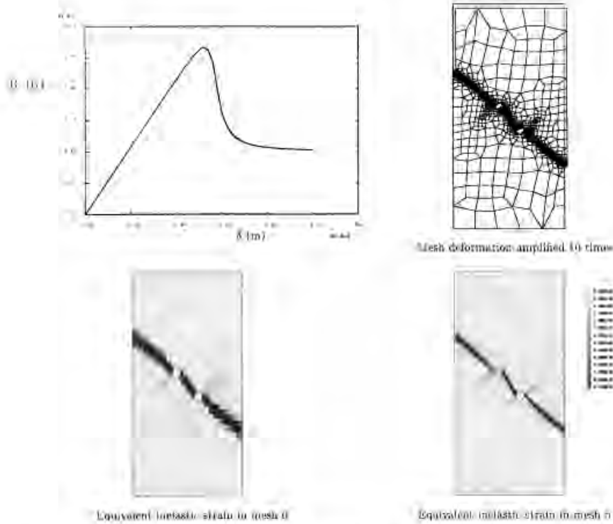
Figure 17. General solution for Example 2a: Reaction versus imposed displacement, deformation of mesh S and inelastic strain contours for meshes 0 and 5 .
