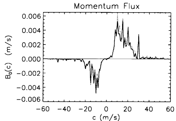
FIG. 11. Zonal intrinsic phase speed spectra of momentum flux at z = 15.875 km for the westerly (solid) and easterly (dotted) QBO cases.
