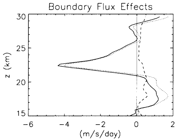
FIG. 9. Same as Fig. 8 but for the easterly shear case. Here the side boundary flux effects (dashed line) are similar to the control case, but small compared to the forcing estimated from the momentum flux convergence, which shows a strong westward peak in the easterly shear at ~22 km.
