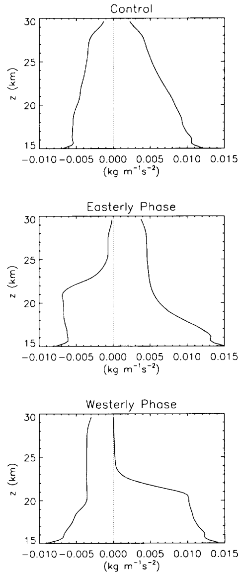
FIG. 7. Three panels showing separate profiles of eastward and westward gravity wave momentum flux averaged over the (x,t) domain for the control (top), easterly QBO (middle), and westerly QBO (bottom) cases.
