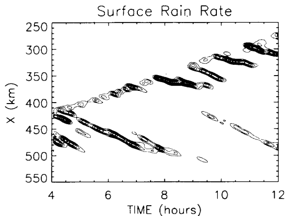
FIG. 4. Contours of surface rainfall vs time and longitude ( x ) for the control simulation. The contour interval is 10^{-4} \text{ g g}^{-1} (rainwater fraction). Intense rainfall is associated with the leading edge of the line (which moves westward) and rearward propagating cells (eastward).
