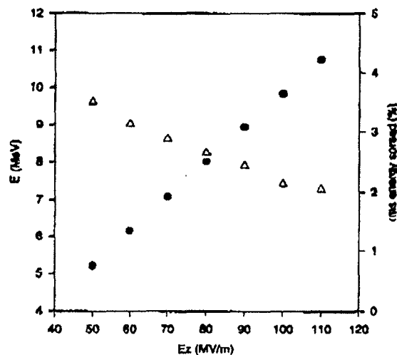
Figure 5. Output energy and energy spread dependence on the cathode field. Solid dots are energy and triangles are energy spread.
