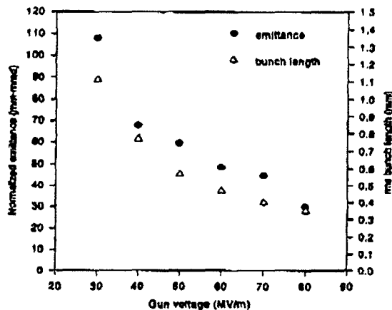
Figure 2. Dependence of the beam parameters at the linac exit on gun axial electrical field. For a 10 nC beam, one can obtain very short and low emittance bunches even at relatively low axial electric field.
