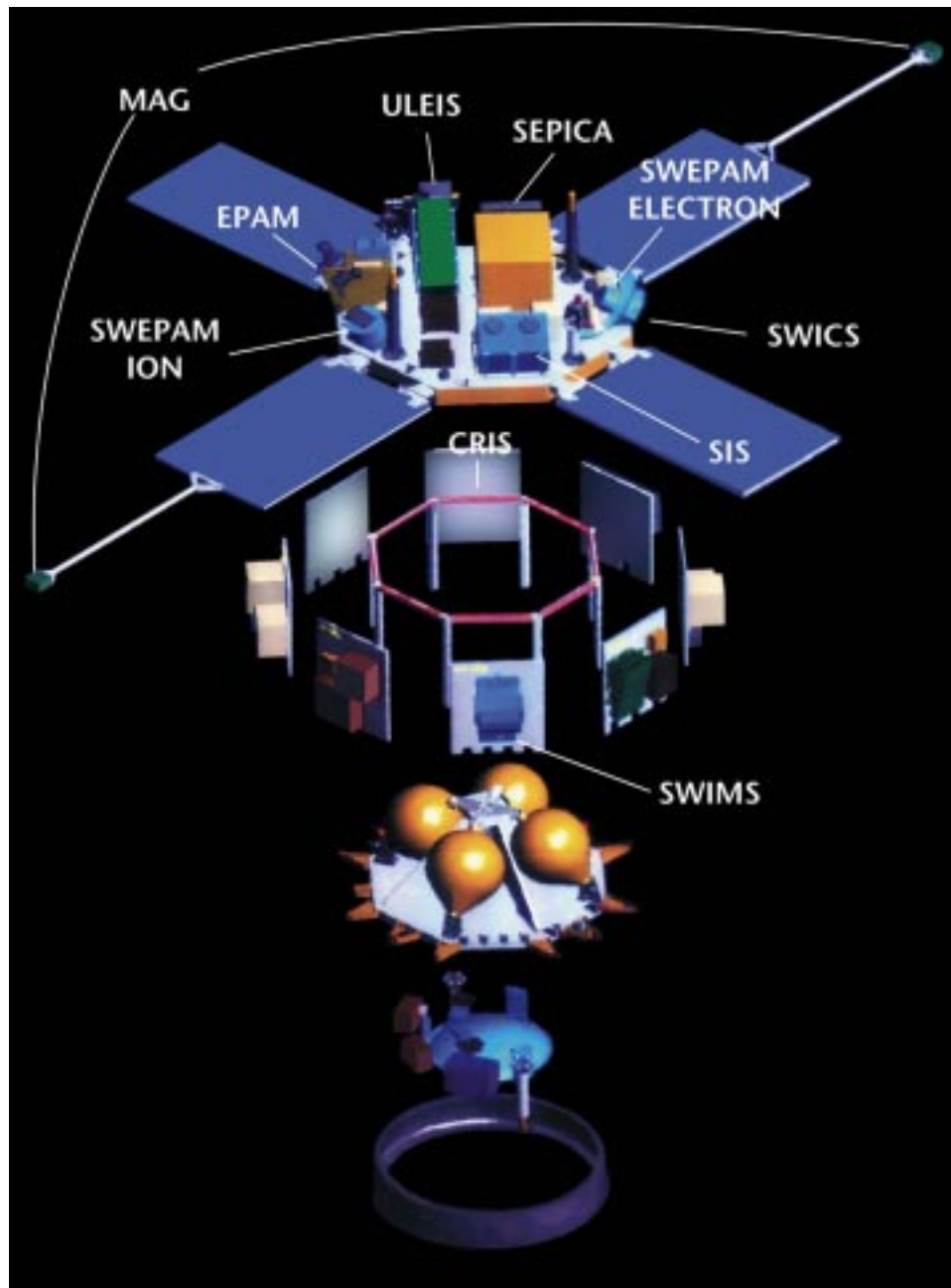
Figure 6. Exploded view of the ACE spacecraft structure. The Z axis is the spin axis of the observatory and will be aligned within 20 degrees of the Earth-Sun line. Six of the scientific instruments are on the +Z (sunward) deck, two are on side-panels, and the ninth is mounted on the Y-axis booms. Only the four propellant tanks of the propulsion subsystem are mounted in the spacecraft interior. The -Z (earthward) deck has the fixed high gain antenna for communication.
