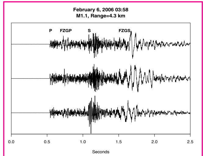
Figure 6. Microearthquake recorded on a seismometer installed in the SAFOD Main Hole located inside the San Andreas fault damage zone about 40 m from an actively slipping trace of the fault. The three velocity seismograms are radial, transverse vertical and transverse horizontal to the source (top to bottom). The high frequency P and S body waves arrive at 0.53 s and 1.07 s, respectively. The dispersed waves following S are fault zone guided S waves (FZGS), which are well known from surface observations. The lower frequency arrival following P is a fault zone guided P wave (FZGP). This is the first known observation of this phase.
