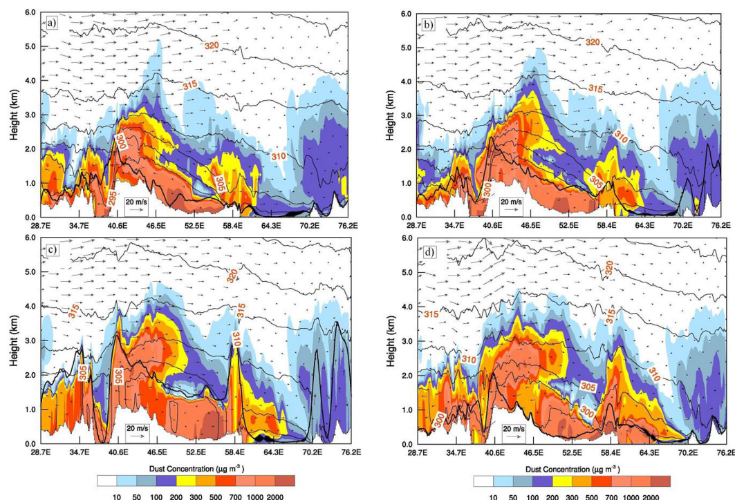
Figure 10. The height longitude cross section along 21.7^{\circ} N showing dust concentration ( \mu\text{g m}^{-3} , shading) and PBL height (km) shown by the black solid line from WRF-Chem on 19 March 2012 at (a) 00:00 UTC, (b) 06:00 UTC, (c) 12:00 UTC, and (d) 18:00 UTC.
