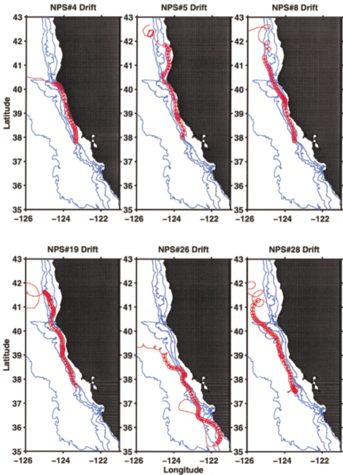
FIG. 6. (Continued) panels the daily positions are indicated by the red symbols. Isobaths for 200, 1000, 2000, and 4000 m are drawn in blue in the individual panels.
