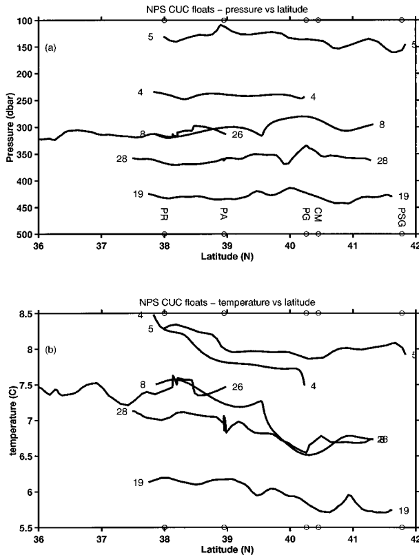
FIG. 12. Pressure (a) and temperature (b) plotted against latitude for the six float segments in the California Undercurrent. Float identification numbers are printed at the beginning and end of each segment. The major coastal promontories indicated in Fig. 7 are again identified by open circles on the latitude axes and labeled with initials.
