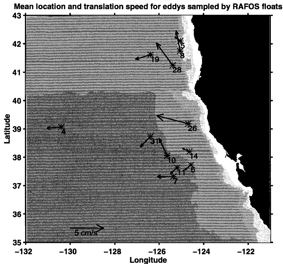
FIG. 13. The mean trajectory of each eddy sampled by the NPS RAFOS floats. The number at the base of each vector is the first float to encounter the eddy as listed in Table 3. The origin of each vector is the location where the eddy was first encountered.
