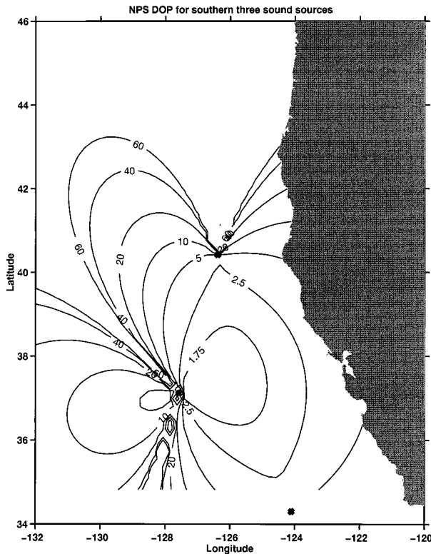
FIG. 2. Dilution of precision (DOP) for the eastern Pacific computed for the geometry of the three southern sound sources (SS 1–3). Units are kilometers. Note that the northern sources were used for navigating floats north of Cape Mendocino, not the sources diagramed in this figure.
