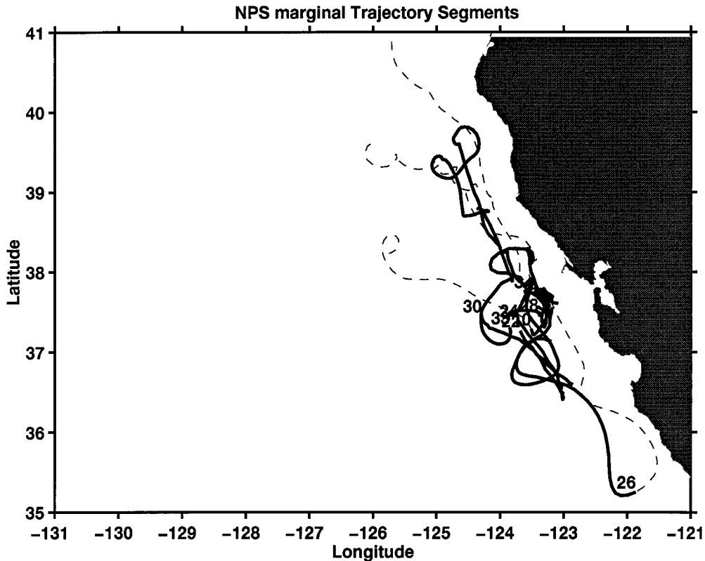
FIG. 8. As in Fig. 6 but for the continental margin flow segment.
