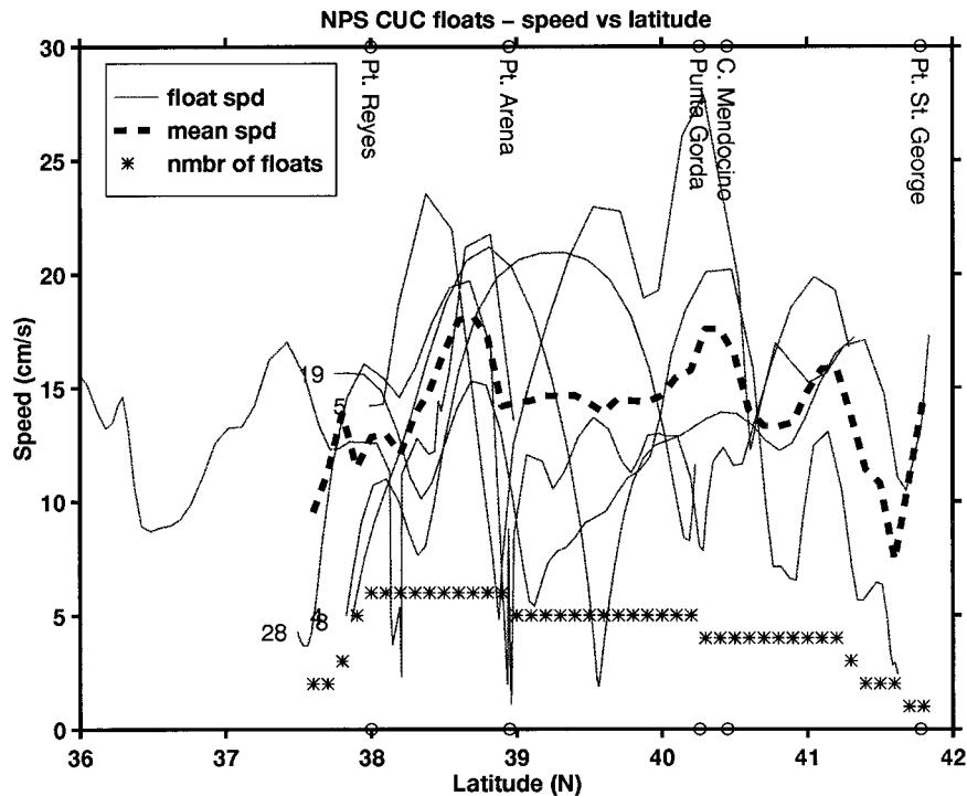
FIG. 7. Plot of float speed ( \text{cm s}^{-1} ) vs latitude for the NPS RAFOs floats caught in the undercurrent. The thin solid lines show individual float daily speeds with float number is given at the start latitude. The thick dashed line is the mean speed. The asterisks give the number of floats used to determine each mean. The major coastal promontories are labeled at the top of the figure and indicated by open circles at the top and bottom of the figure.
