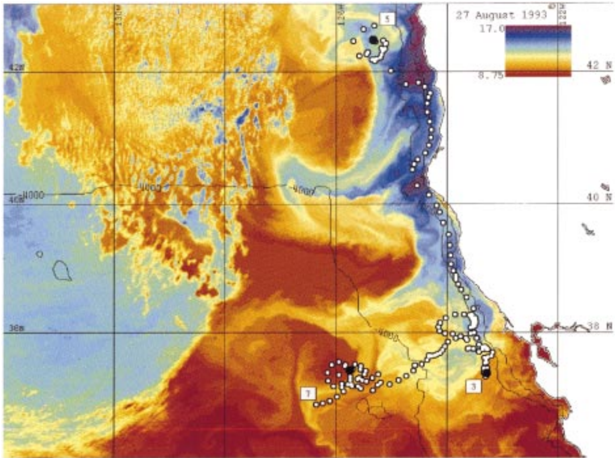
FIG. 10. Satellite imagery for 27 August 1993, with float trajectories for NPS 3, 5, and 7 superimposed. The dots are the daily interpolated float positions. The float position on the day of the satellite overpass is marked by a large black dot.
