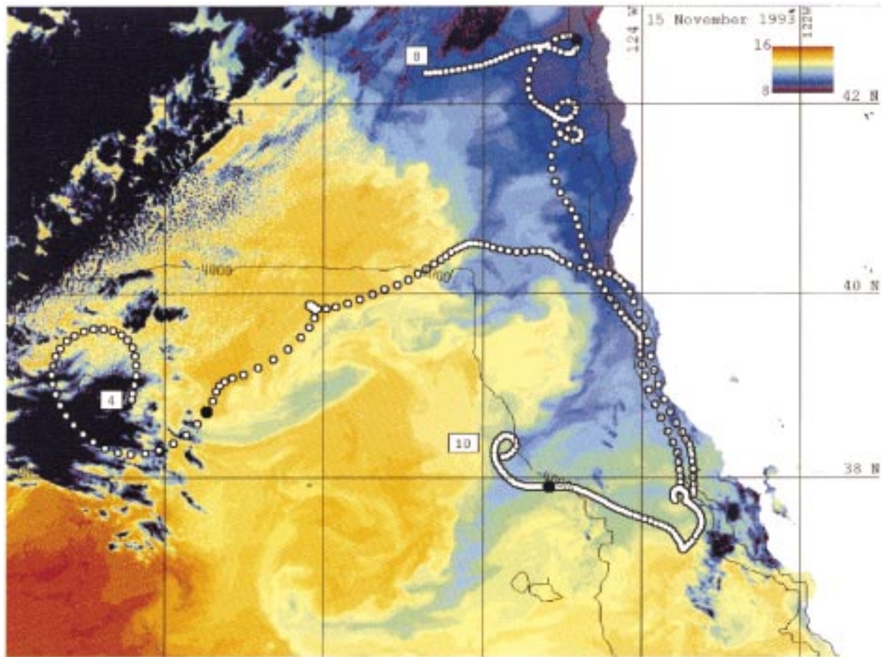
FIG. 11. Satellite imagery for 15 November 1993, with float trajectories for NPS 4, 8, and 10 superimposed. The dots are the daily interpolated float positions. The float position on the day of the satellite overpass is marked by a large black dot.
