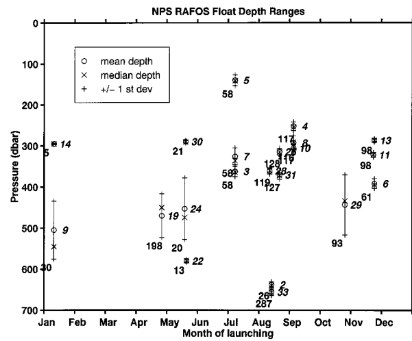
FIG. 4. Depth range (mean, median, and standard deviation) of the NPS RAFOS floats. The NPS float number is in italics to the right of the mean depth, and the number of daily pressure values used to determine the statistics is below the variance bar. The depth for NPS14 was estimated from the temperature record. The depth variability is placed at the launch date for each float.
