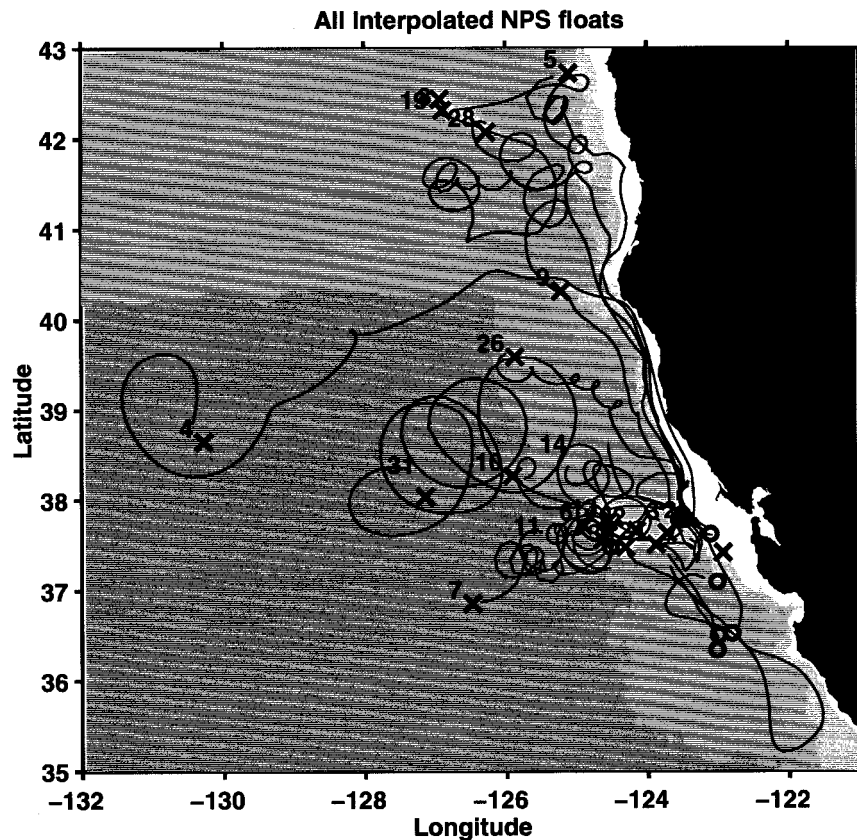
FIG. 5. Ensemble spaghetti diagram showing the smoothed subsurface trajectories of all the NPS RAFOS floats. The launch sites are indicated by circles, and the location where each float surfaced is indicated with an "x." The float number is placed at the surfacing location. Depth shading is keyed to isobaths at 200, 1000, 2000, and 4000 m.
