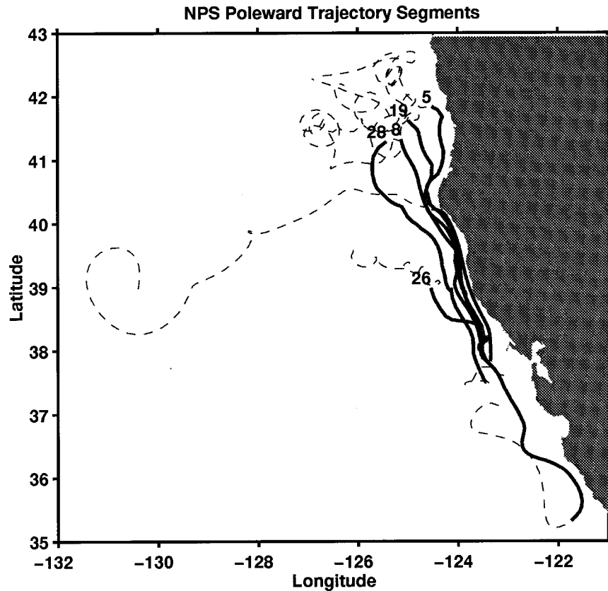
FIG. 6. Ensemble and individual spaghetti plots for the California Undercurrent flow regime. The undercurrent segment is drawn as a heavy line in the ensemble panel. In the individual
