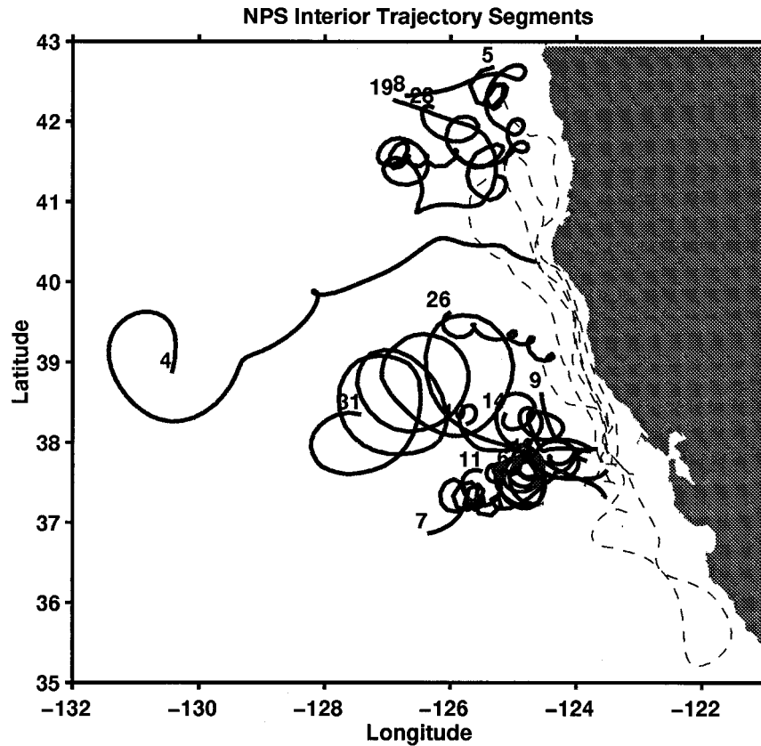
FIG. 9. As in Fig. 6 but for the interior Pacific flow segment.
