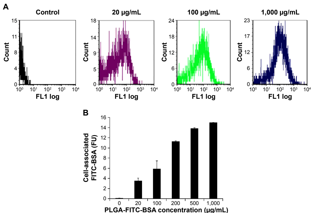
Figure 2 Cellular uptake of BSA encapsulated into PLGA NPs analyzed by flow cytometry.
