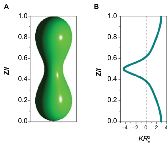
Figure 5 The Gaussian curvature, K . For the membrane shape shown in (A) we plotted the variations of normalized Gaussian curvature, KR_0^2 , along the symmetry axis-z shown in (B) . At the neck, K is negative; therefore, it attracts defects with a negative topological charge. On the other hand, defects with a positive topological charge tend to assemble at regions where K > 0 . The membrane shape was calculated for \langle h \rangle = 1.275 and \nu = 0.695 . l stands for the length of the membrane along the z axis and R_0 = (A/4\pi)^{1/2} , where A is the membrane area.
