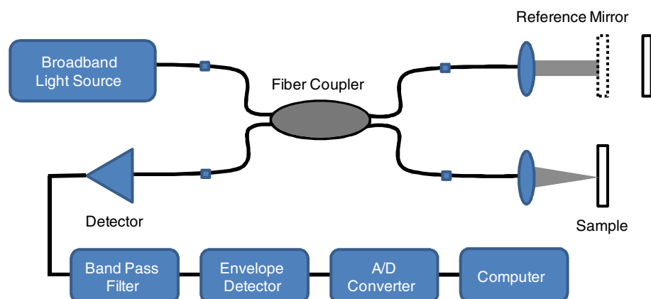
Fig. 1. Schematic representation of a fiber based time domain OCT system. The Michelson interferometer is implemented using a fiber-optic coupler. Light from the low-coherence source is split and sent to a sample arm with a beam delivery instrument and a reference arm with an optical path-length scanner. Reflected light from both arms are combined and is detected with a photodiode in the output of the interferometer.
