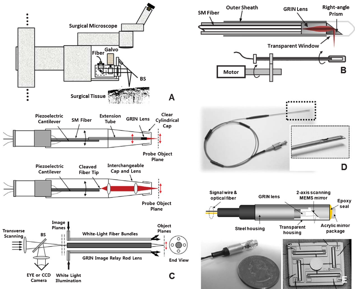
Fig. 2. Beam delivery instruments. Various OCT imaging probe can be implemented which include (A) surgical and research microscope, (B) fiber-optic catheter, (C) hand-held probes and laparoscope, (D) optical needle-probe, (E) 2-D MEMS scanner based endoscopic probe.
