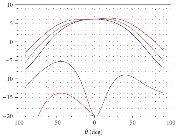
FIGURE 8: Simulated radiating pattern in transmit.
