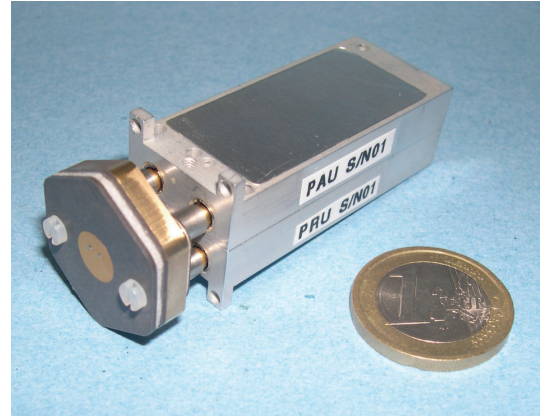
FIGURE 9: Tx/Rx active module connected to the radiating element.
