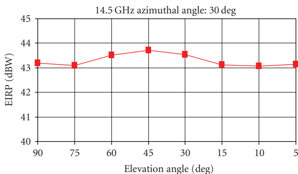
FIGURE 18: EIRP versus elevation angle over the horizon.
