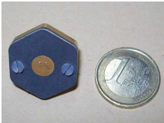
FIGURE 5: Radiating element prototype.
