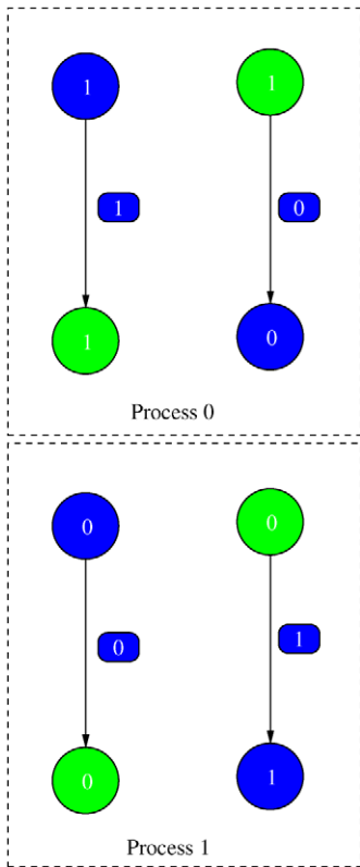
Fig. 5. Partition point Overlap, with dark partition points, light process ranks, and arrow labels representing remote points. The send Overlap is on the left, and the receive Overlap on the right.
