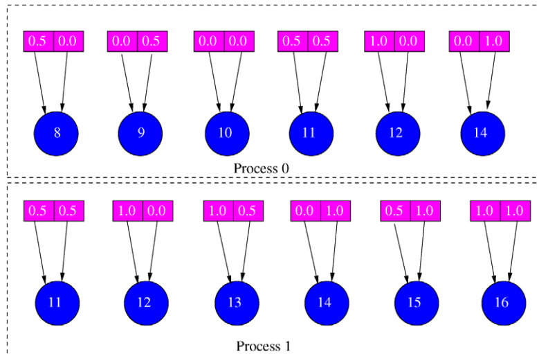
Fig. 17. Distributed coordinate Section.
