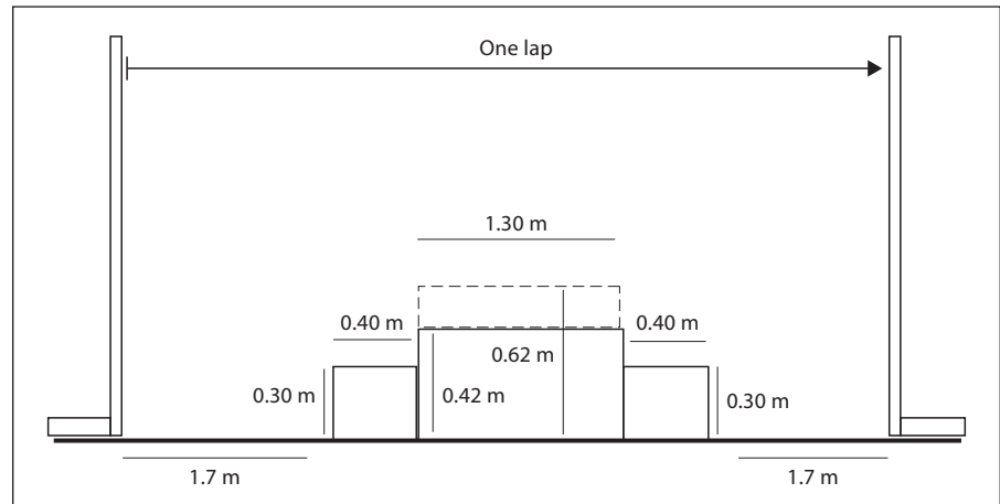
Fig. 1. Set-up equipment for the 5MPT. The height of the central box for the old adults was 0.42 m and for the young adults 0.62 m. The total lap distance was 5.5 m.
