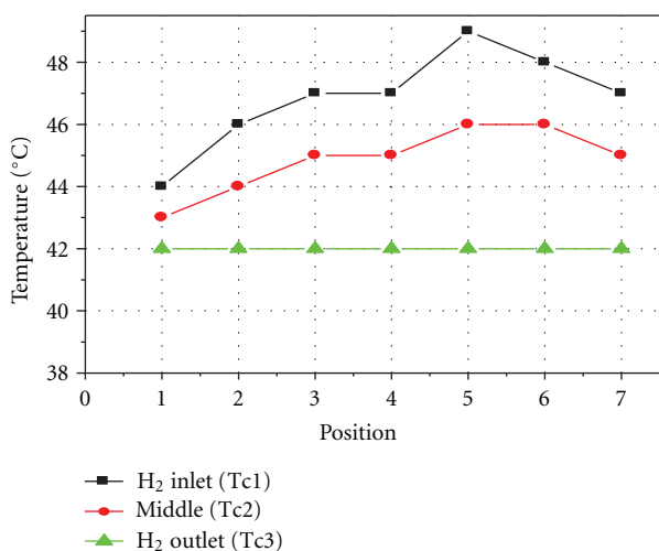
FIGURE 7: Temperature variation within the stack.
