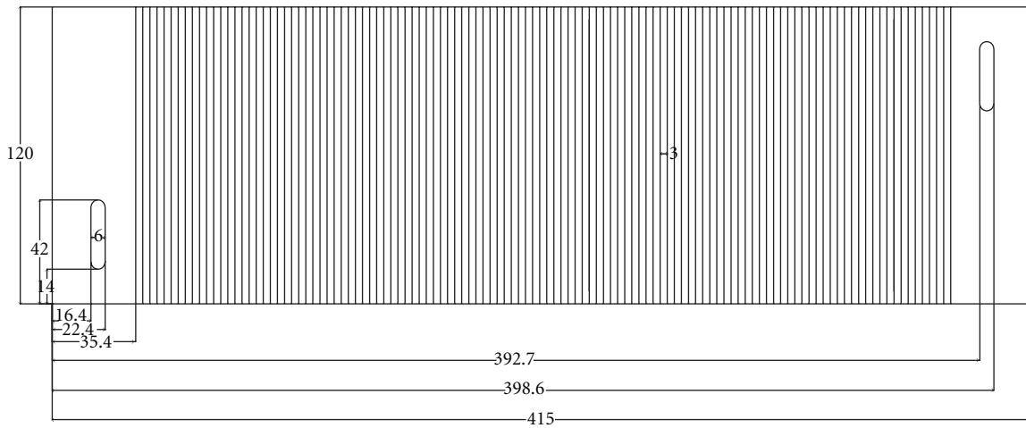
FIGURE 2: Flow field design for air supply/coolant.
