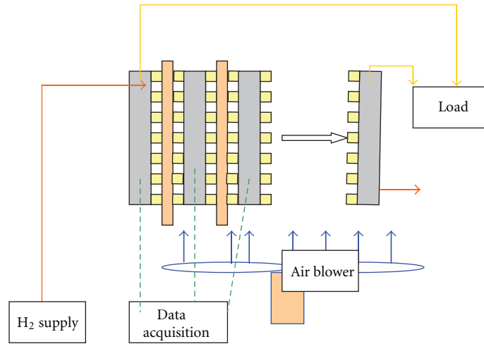
FIGURE 1: Schematic of stack and test apparatus.
