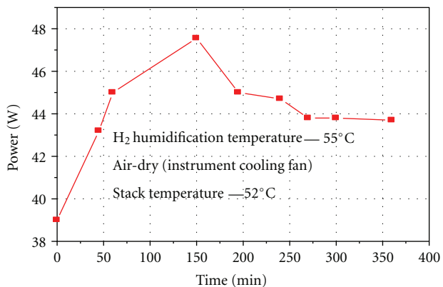
FIGURE 6: Stability of the stack performance.
