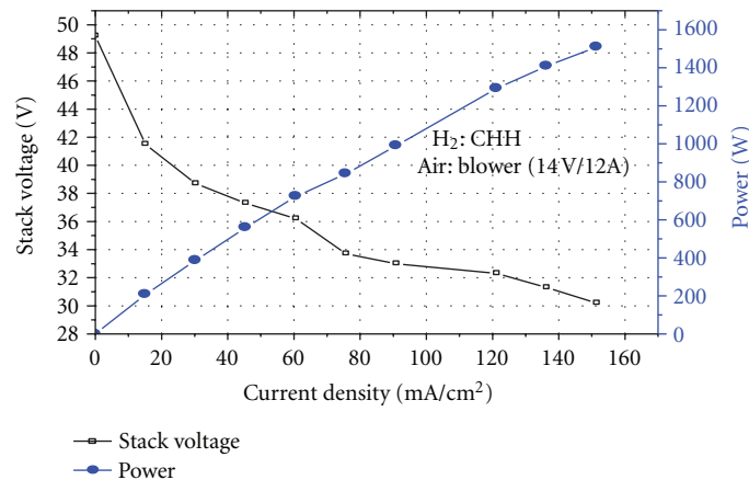
FIGURE 11: 1.5 kW fuel cell performance curve.
