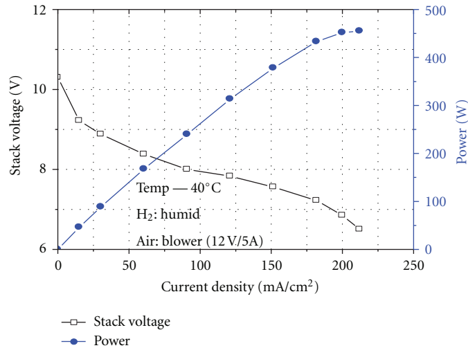
FIGURE 10: 500 watt fuel cell performance curve.
