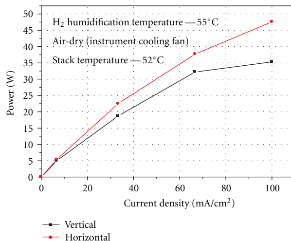
FIGURE 5: Fuel cell performance due to stack orientation.
