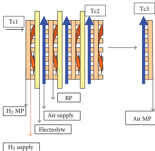
FIGURE 9: Schematic of fuel cell stack assembly.
