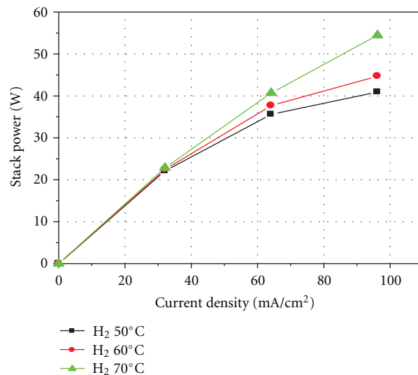
FIGURE 4: Fuel cell performance at different humidity.
