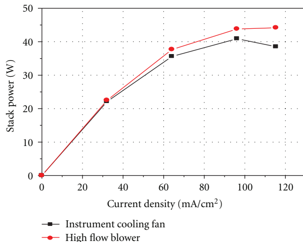
FIGURE 8: Fuel cell performance due to different air-moving device.
