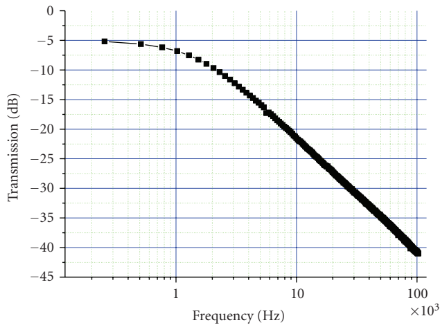
FIGURE 3: The measured transmission of the 2m-long resistive wire pair.
