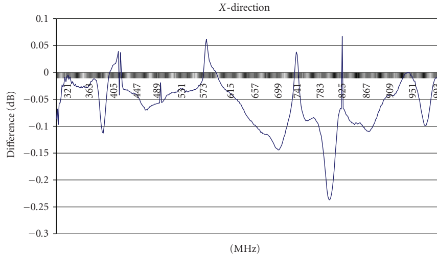
FIGURE 2: The difference in the transmission of the GTEM cell with and without loading in the screen printed resistive lines.
