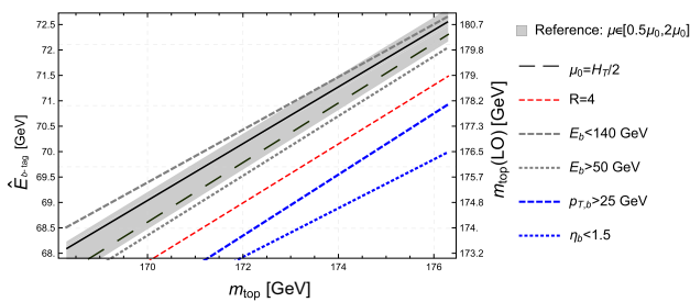
Fig. 6 Prediction of the fitted energy peak as a function of m_t , as obtained from: fitting the part of the energy spectrum 45 GeV < E_{b\text{-tag}} < 140 GeV (gray thick short dashed); 50 GeV < E_{b\text{-tag}} < 160 GeV (gray thick dotted), both under the selection criteria in (8); changing the selections to p_{T,b} > 25 GeV (blue thick dashed); changing the selections to |\eta_b| < 1.5 GeV (blue thick dotted). The red thin dashed line shows the result for the calculation with the anti- k_T jets made with size parameter R = 0.4 . For reference the band and the central prediction solid line of Fig. 3 are reported, along with the central prediction for dynamical scale H_T/2 from the same figure. To ease the reading of the resulting uncertainty on m_t , along the right vertical axis we give the top quark mass corresponding to the \hat{E}_{b\text{-tag}} according to the LO formula in (1)
