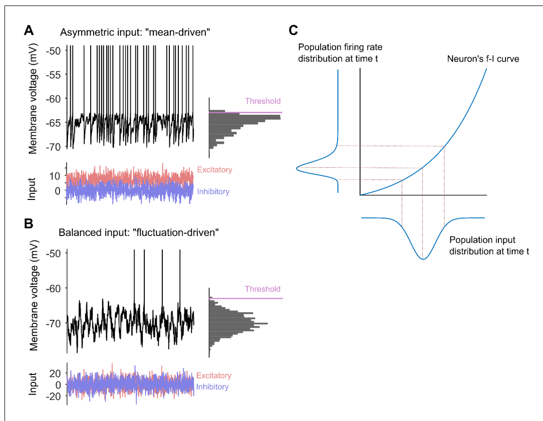
Figure 1. Long-tailed distributions and balanced networks. (A) When a single neuron receives more excitatory input (red) than inhibitory input (blue), its membrane voltage (black line) spikes regularly. In this "mean-driven" model the membrane voltage spends much of its time at or near the spiking threshold (see histogram on right), and spiking is driven by the difference between the means of the excitatory and inhibitory inputs. However, most neurons do not spike as rapidly or regularly as predicted by the "mean-driven" model. (B) The theory of balanced networks proposes that the inhibitory and excitatory inputs to a neuron have approximately the same mean and the same variance. Consequently, spiking is driven by random fluctuations in the inputs, when the excitatory input briefly exceeds the inhibitory input. A signature of this "fluctuation-driven" regime is that the distribution of the membrane voltage is approximately Gaussian (histogram). Fluctuation-driven neurons spike slowly and irregularly, similar to the majority of the neurons in the cortex. (C) The relationship between the input to a neuron (blue curve below the x-axis) and its spiking or firing rate (blue curve to the left of the y-axis) is described by a firing rate versus input ( f-i ) curve. In 2011 Roxin et al. predicted that an expansive f-i curve (see main text) would convert a Gaussian input into a long-tailed distribution of firing rates in the fluctuation-driven regime. Moreover, according to this theory, if each neuron has a Gaussian input, then the overall population of neurons will also have a Gaussian input, and if each neuron has an expansive f-i curve in the fluctuation-driven regime, then the output of the population will be long-tailed.
