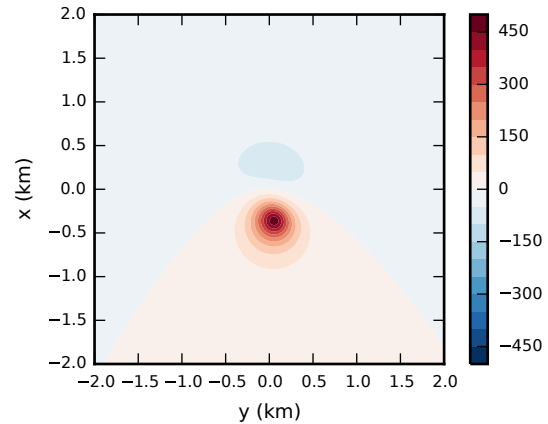
Figure 5. Total-field anomaly (in nT) produced by the synthetic orebody defined in Table 2. The synthetic data are calculated on a regular grid of 100 \times 100 points at the constant vertical coordinate z = 0 m.
