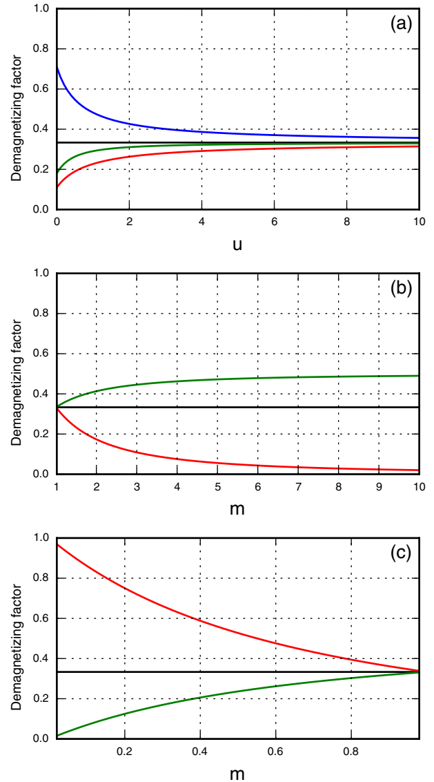
Figure 2. (a) Comparison between the demagnetizing factors \tilde{n}_{11}^{\dagger} (in red), \tilde{n}_{22}^{\dagger} (in green) and \tilde{n}_{33}^{\dagger} (in blue) produced by 100 triaxial ellipsoids with semi-axes a = a_0 + u b_0 , b = b_0 + u b_0 and c = c_0 + u b_0 , where 0 \leq u \leq 10 and b_0 = 700 m. The demagnetizing factors were calculated by using Eqs. (25), (26) and (27). (b) Comparison between the demagnetizing factors \tilde{n}_{11}^{\dagger} (in red) and \tilde{n}_{22}^{\dagger} (in green) produced by 100 prolate ellipsoids with semi-axes a = m b_0 and b = b_0 , where 1.02 \leq m \leq 10 and b_0 = 1000 m. The demagnetizing factors were calculated by using Eqs. (30) and (31). (c) Comparison between the demagnetizing factors \tilde{n}_{11}^{\dagger} (in red) and \tilde{n}_{22}^{\dagger} (in green) produced by 100 oblate ellipsoids with semi-axes a = m b_0 and b = b_0 , where 0.02 \leq m \leq 0.98 and b_0 = 1000 m. The demagnetizing factors were calculated by using Eqs. (32) and (33). The horizontal black line represents the value 1/3 .
