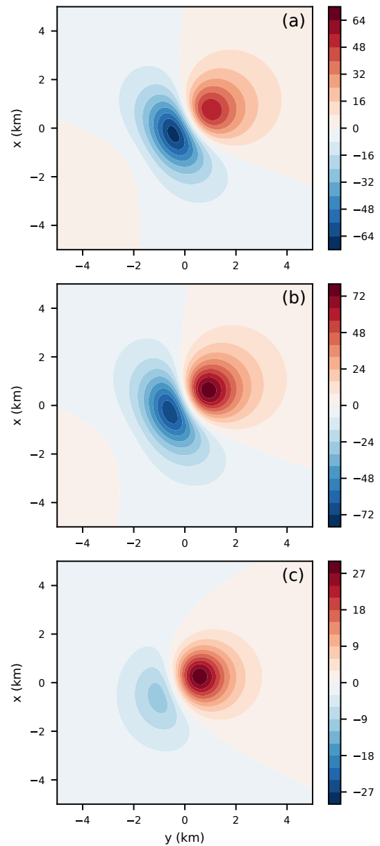
Figure 4. Total-field anomalies (in nT) produced by (a) Ellipsoid 1 and (b) Ellipsoid 2, both defined in Table 1. The synthetic data produced by these confocal ellipsoids were calculated on a regular grid of 200 \times 200 points at the constant vertical coordinate z = 0 m. These data were calculated with a uniform inducing field which is oblique to the semi-axes of the confocal ellipsoids. (c) Difference between the total-field anomalies shown in (b) and (a).
