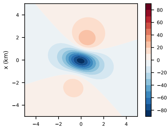
Figure 3. Total-field anomaly (in nT) produced by the synthetic bodies Ellipsoid 1 and Ellipsoid 2, both defined in Table 1. The synthetic data produced by these confocal ellipsoids were calculated on a regular grid of 200 \times 200 points at the constant vertical coordinate z = 0 m. These data were calculated with a uniform inducing field parallel to the semi-axis a of the confocal ellipsoids.
