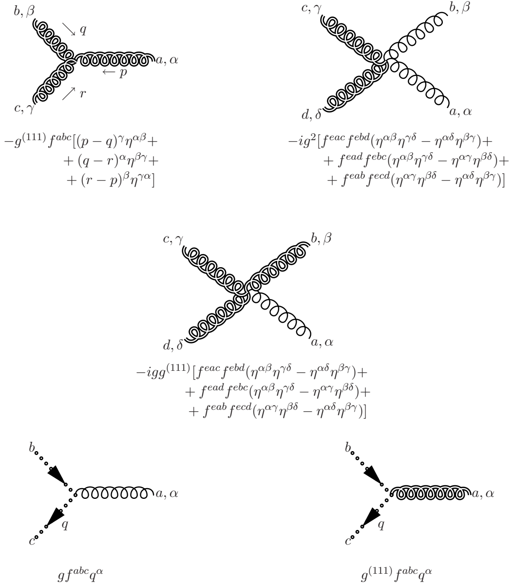
Figure 1. Feynman rules required to evaluate the diagrams relevant for the gg \rightarrow g_{\text{KK}} process. The KK gluon is denoted by a double gluon line, and the KK ghost is denoted by lines of circles.
