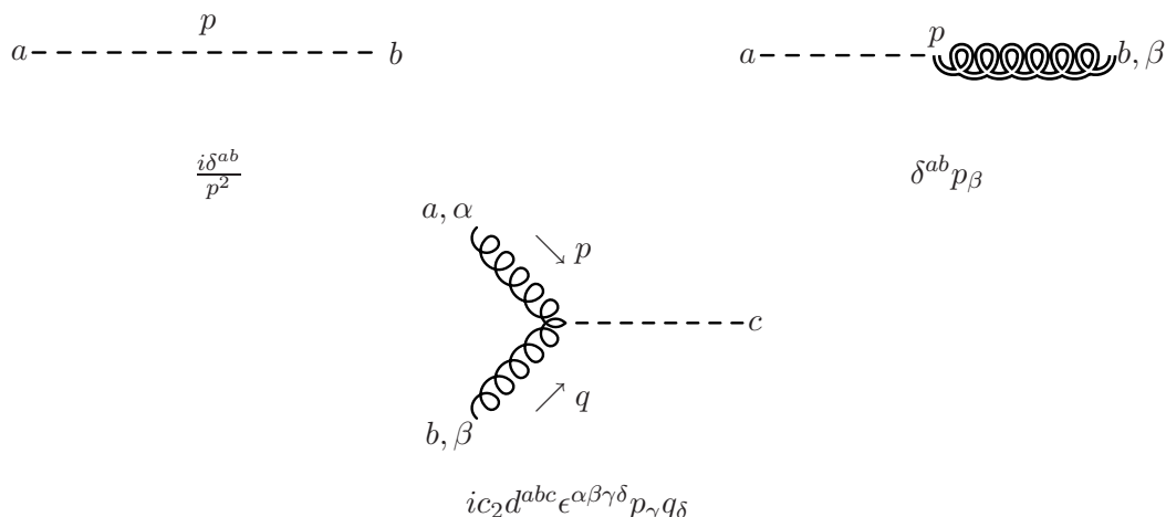
Figure 5. Additional relevant non-zero Feynman rules for gauges with A_4 \neq 0 .
