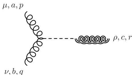
Figure 6. Additional Feynman diagram for the process gg \rightarrow g_{\text{KK}} for gauges with A_4 \neq 0 .
