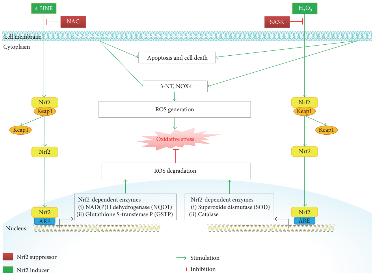
FIGURE 1: Schematic diagram of Nrf2 signaling and regulation in the corneal epithelial cells. 4-HNE or H 2 O 2 induces excessive ROS generation (by upregulation of 3-NT, NOX4 protein expression), leading to oxidative stress in the cultured HCE cells and resulting in cell apoptosis and death of corneal epithelial cells. 4-HNE activates Nrf2/ARE-controlled antioxidant enzyme (NQO1 and GSTP) transcription, which facilitates ROS degradation. On the other hand, H 2 O 2 decreases Nrf2/ARE-controlled SOD and catalase transcription, leading to ROS degradation suppression. NAC serves as an antioxidant by antagonizing 4-HNE overexpression and reversing the cell viability of HCE cells. SA3K blocks H 2 O 2 -induced ROS, 3-NT, and NOX4 overexpression and upregulates ROS degradation by activating Keap1-Nrf2-ARE pathway.
