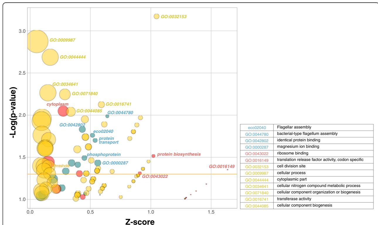
Fig. 3 Differential enrichment of GO, KEGG and UP_KEYWORDS functional terms in three groups of genes (Fig. 2): S_{high} and/or E_{high} phenotype (Groups #1–6, yellow circles), predominant S_{low} phenotype (Groups #7–11, red circles) and predominant E_{low} phenotype (Groups #12–16, blue circles). Axes represent enrichment p -value ( \log_{10} transform, y-axis) and the enrichment’s z-score (x-axis). Functional terms selected for differential enrichment (legend) have very significant score ( >2 ) or p -value ( <0.1 ), or pass a \text{Log}_{10}(p) \leq 1.3 and z \geq 0.5 combined threshold
