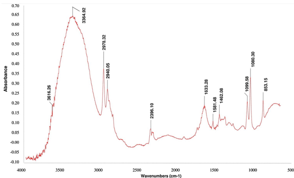
Fig. 8 FTIR analysis of biosynthesized AgNPs
