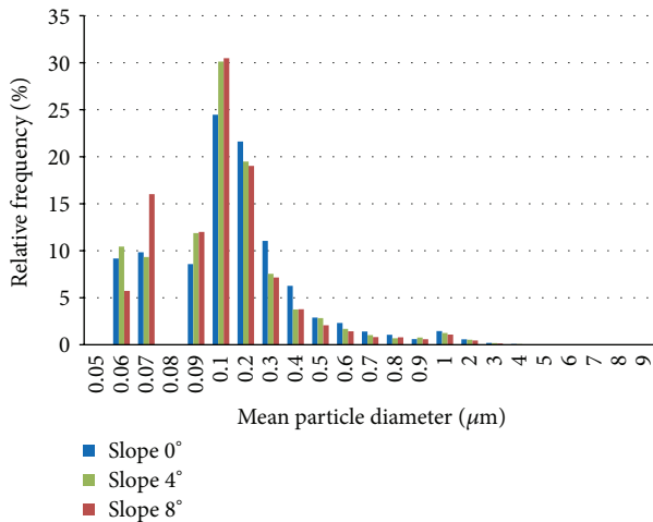
FIGURE 6: Frequency distribution of wear particles of the mean diameter for the different slope angles generated between 4.5 and 5.0 million cycles.
