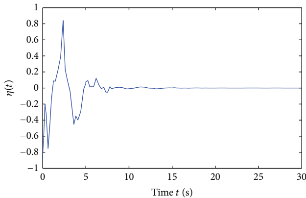
FIGURE 3: Estimated signals error \eta(t) = z(t) - \tilde{z}(t) .
