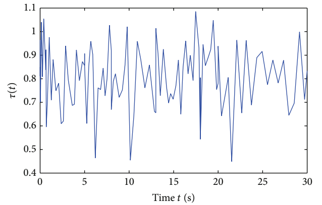
FIGURE 2: Interval time-varying delay.
