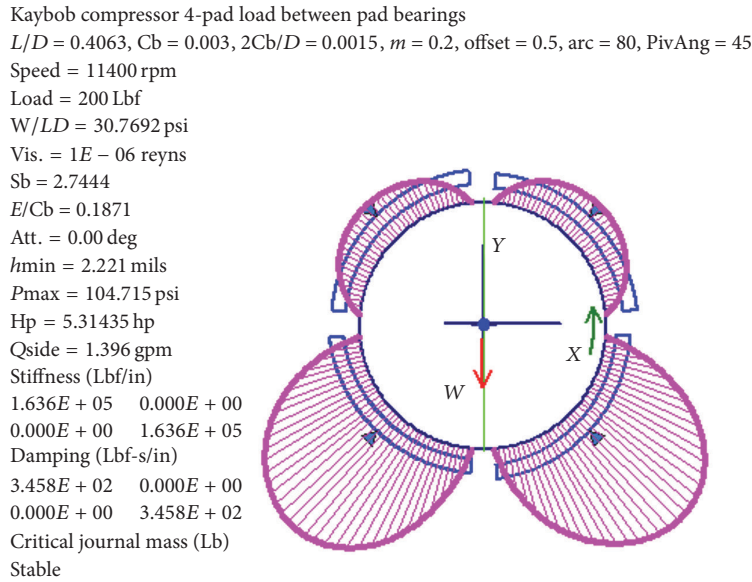
FIGURE 18: Results of the four-pad bearing analysis.
