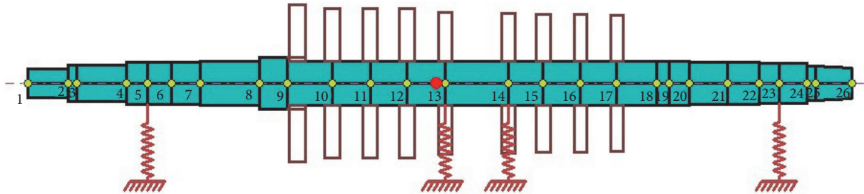
FIGURE 5: Kaybob 9-stage compressor model with aerodynamic cross-coupling at stations 13 and 14.
