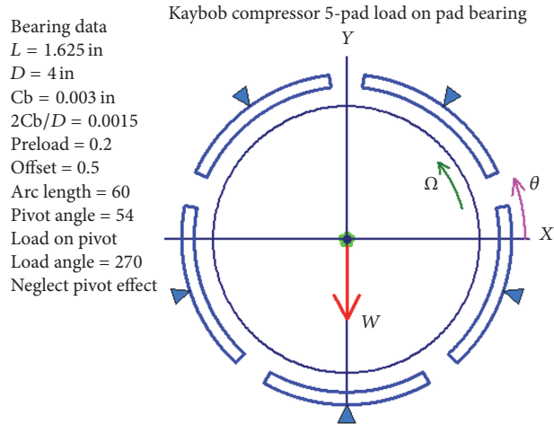
FIGURE 10: Original compressor bearing design.
