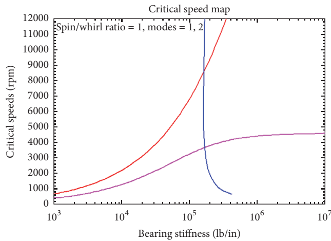
FIGURE 6: Compressor critical speed map.
