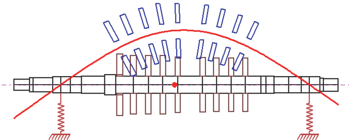
FIGURE 7: First bending mode of the compressor.
