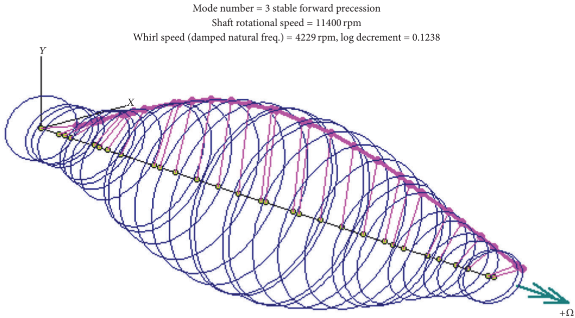
FIGURE 29: Stability analysis of the new rotor design with the original five-pad LOP bearings.
