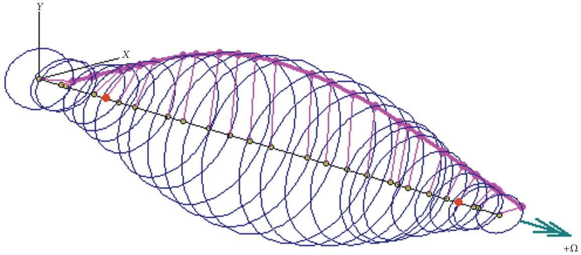
FIGURE 25: Stability analysis of the nongrooved squeeze film damper supported system.
