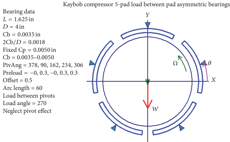
FIGURE 14: Asymmetric bearing model.
