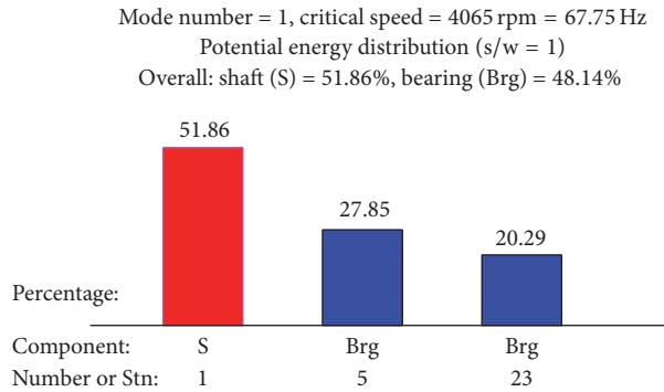
FIGURE 13: First mode shaft and bearings energy distribution with the original bearing design.
