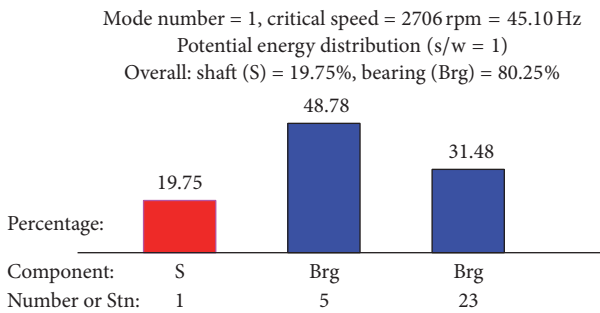
FIGURE 23: Energy distribution in the shaft and bearings for the improved four-pad bearing design.
