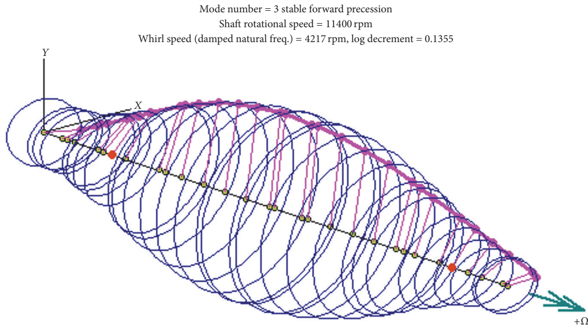
FIGURE 30: Stability analysis of the new rotor design with the original bearing and a long squeeze film damper.
