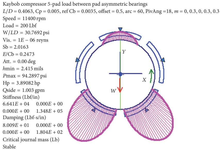
FIGURE 15: Results for the asymmetric bearing.
