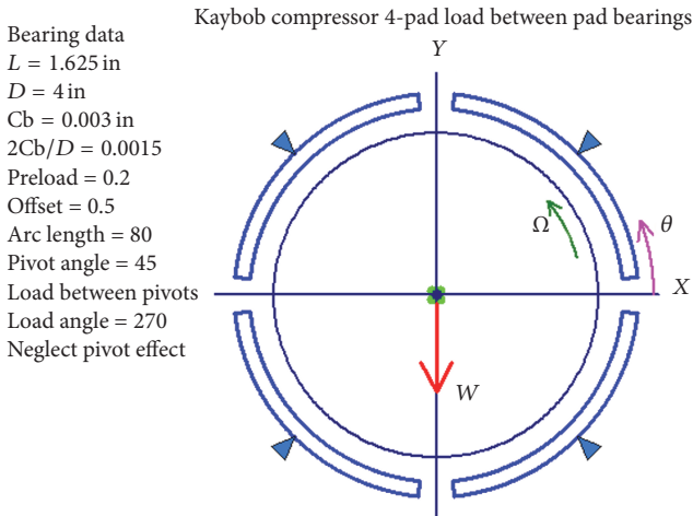
FIGURE 17: Initial four-pad bearing design.
