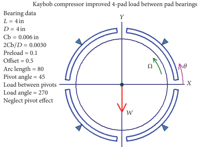
FIGURE 20: Improved four-pad bearing design.
