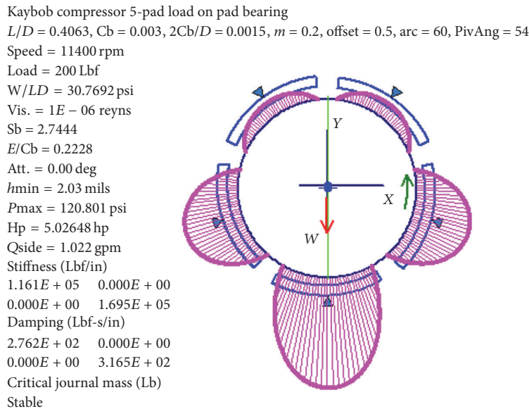
FIGURE 11: Original compressor bearing analysis results.
