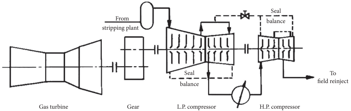
FIGURE 1: Kaybob compressor train schematic from Smith [1].
