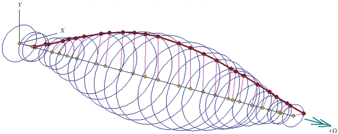
FIGURE 19: Stability results for a four-pad bearing design.
