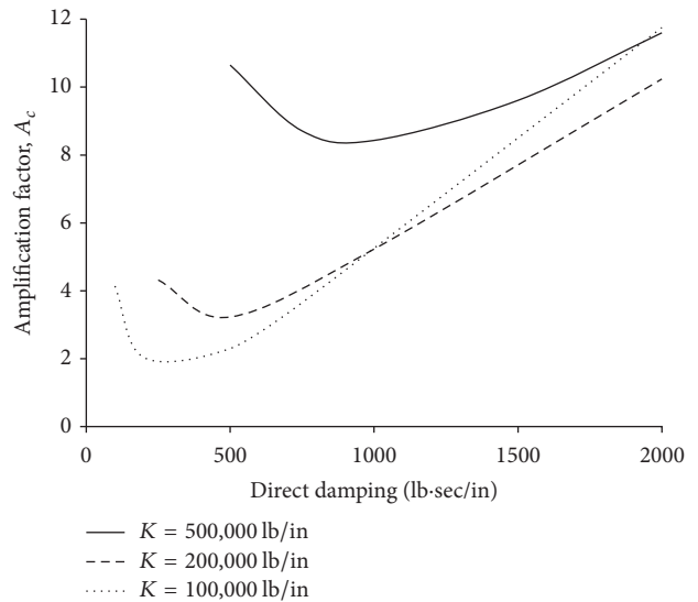
FIGURE 9: Amplification factors of the first bending mode.
