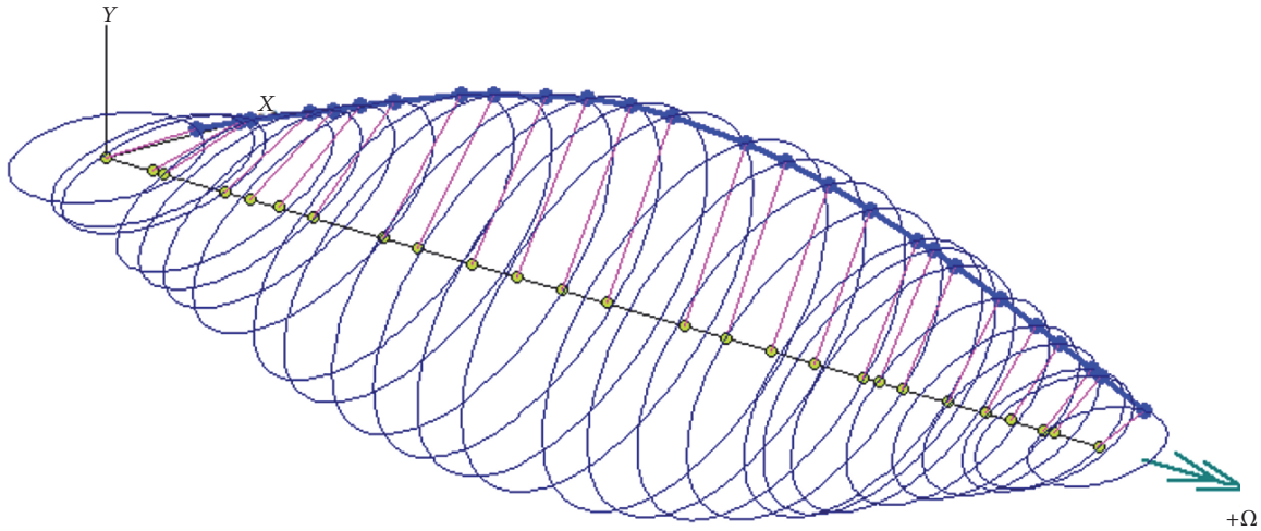
FIGURE 16: Stability results for the asymmetric bearing.
