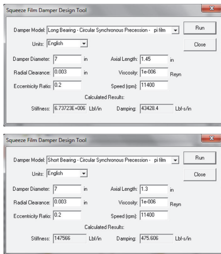
FIGURE 24: Nongrooved and grooved squeeze film damper analysis.
