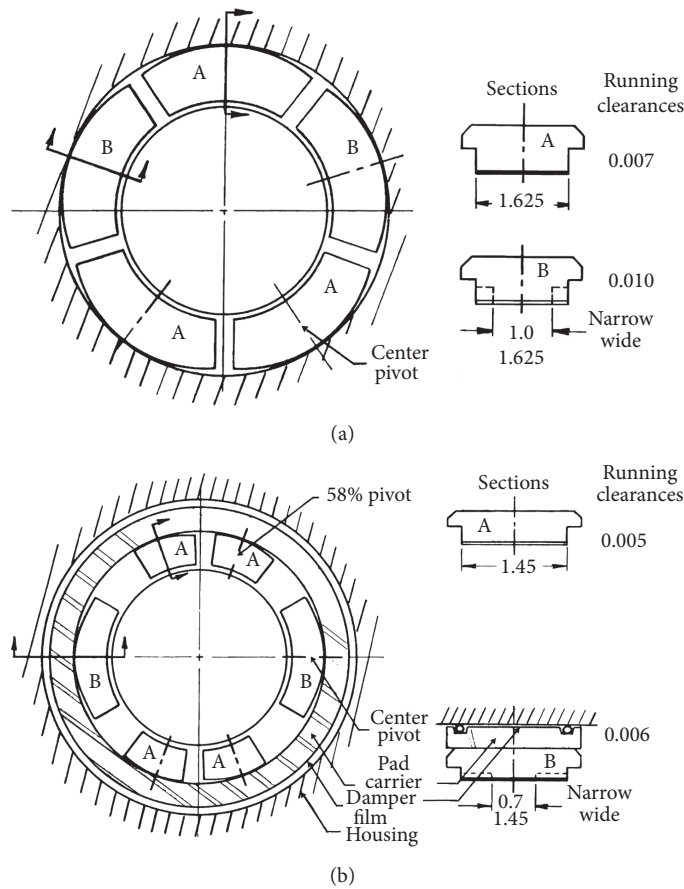
FIGURE 3: (a) Asymmetric tilt pad bearing from Smith [1]. (b) Squeeze film damper design from Smith [1].
