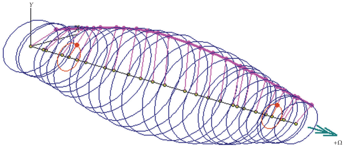
FIGURE 26: Stability analysis of the grooved squeeze film damper supported system.
