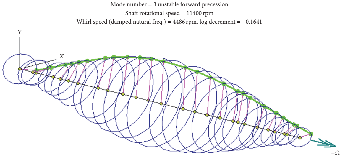
FIGURE 12: Stability results for the original bearing design.
