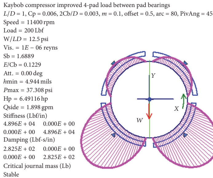
FIGURE 21: Analysis of the improved four-pad bearing.
