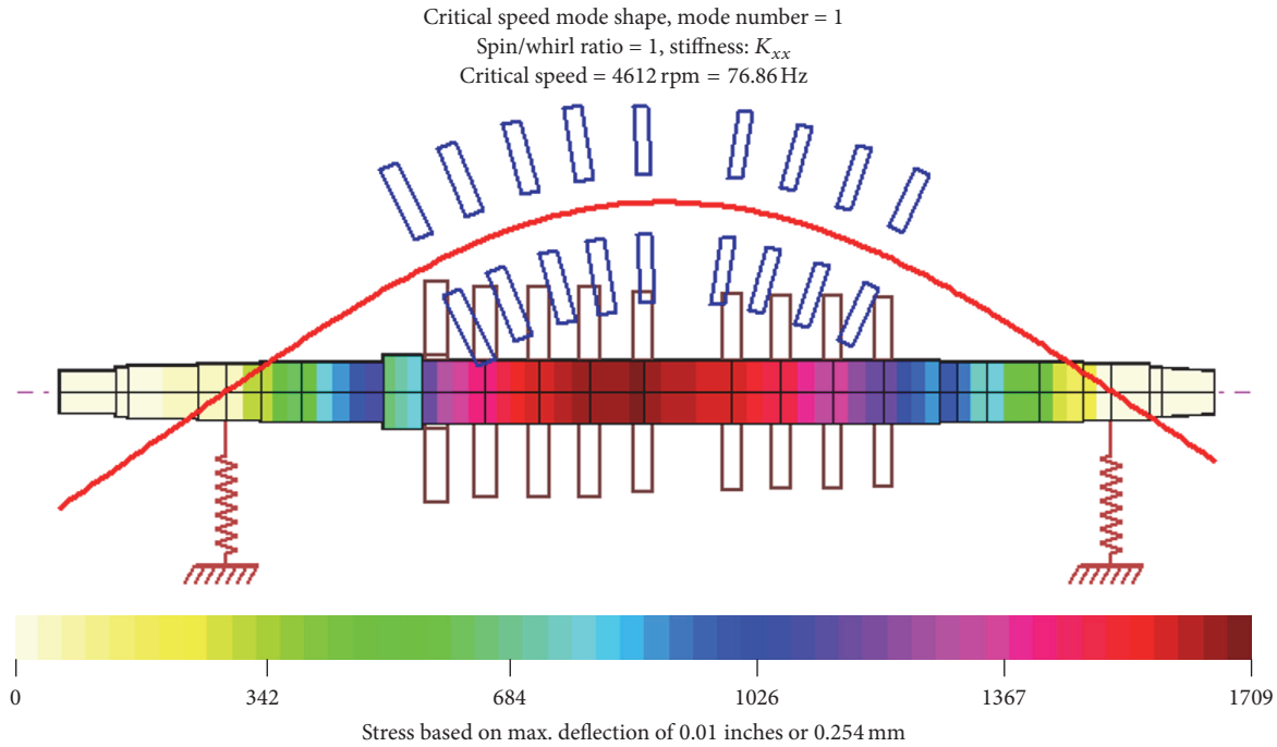
FIGURE 8: Shaft modal stresses of the first bending mode.
