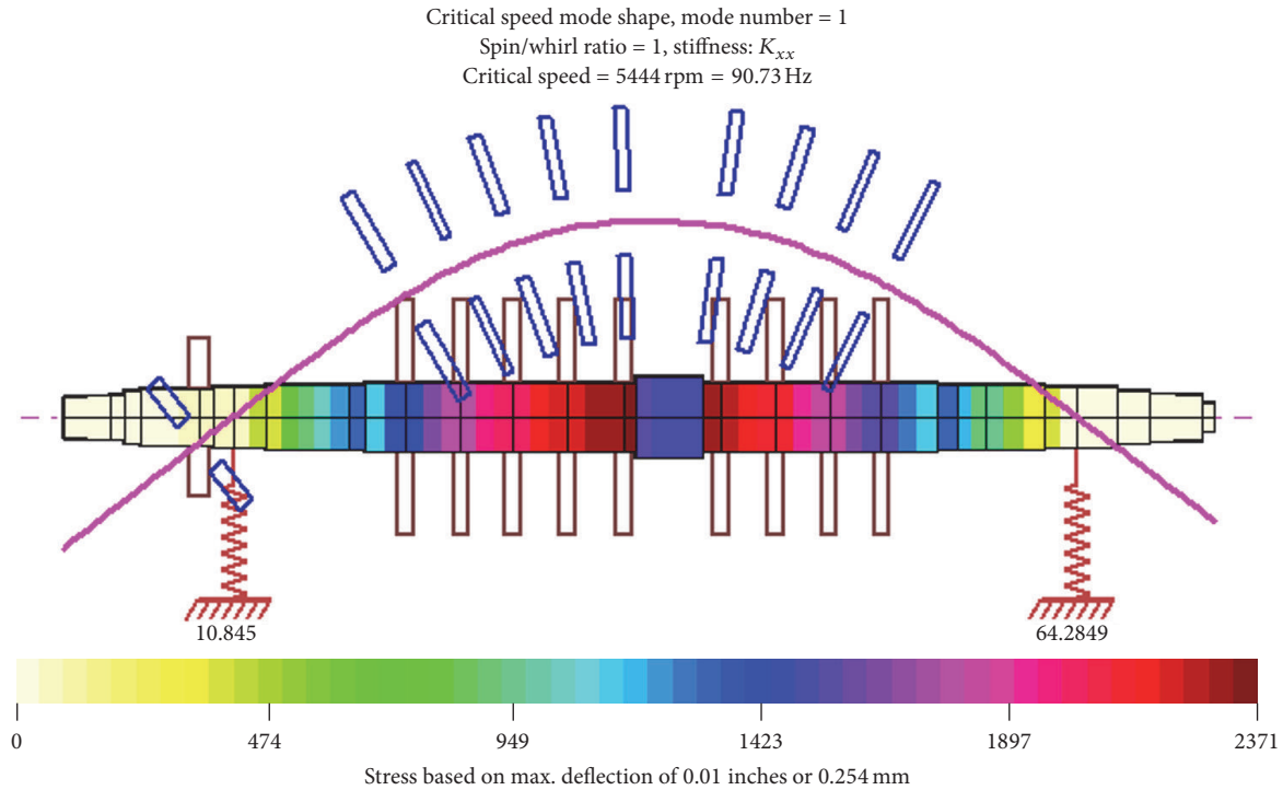
FIGURE 28: Shaft modal stresses of the first bending mode.
