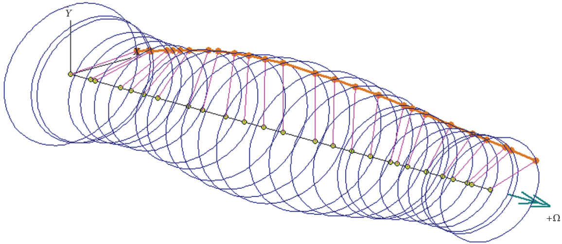
FIGURE 22: Stability analysis of the improved four-pad bearing.
