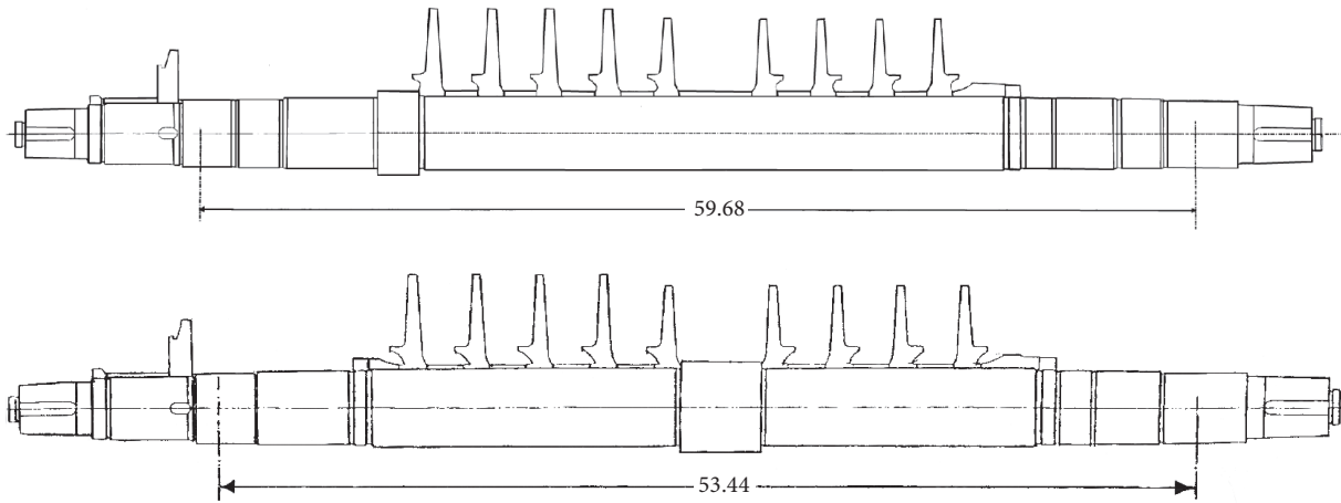
FIGURE 4: Rotor redesign from Smith [1].
