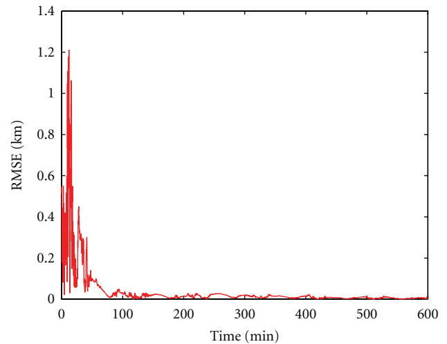
FIGURE 7: EKF RMSE.
