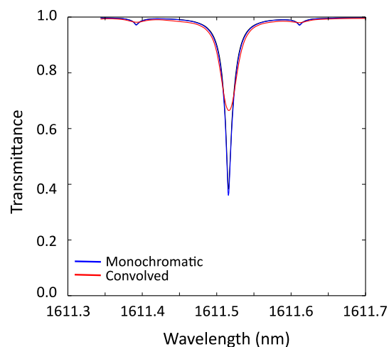
Fig. 6 Effect of instrument line broadening: The 1.5-GHz heterodyne bandwidth causes the lineshape to be broadened. For this reason, prior to fitting data to calculations, we convolve the calculated transmitted lineshape with the instrument response as shown in this plot
