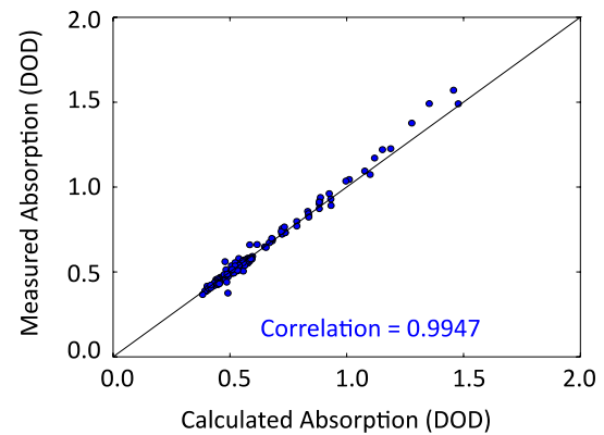
Fig. 8 Baseline instrument performance—the absorption measured by the Mini-LHR is compared against calculations based on the solar zenith angle (for fixed CO 2 ) for all cloud-free data taken at MLO in May 2013. The high correlation coefficient shows that the change in absorption due to change in optical path length is completely captured by the LHR. This is a prerequisite for CO 2 concentration measurements. The absorptions are expressed in terms of the differential optical depth (DOD) between line center and off-line points
