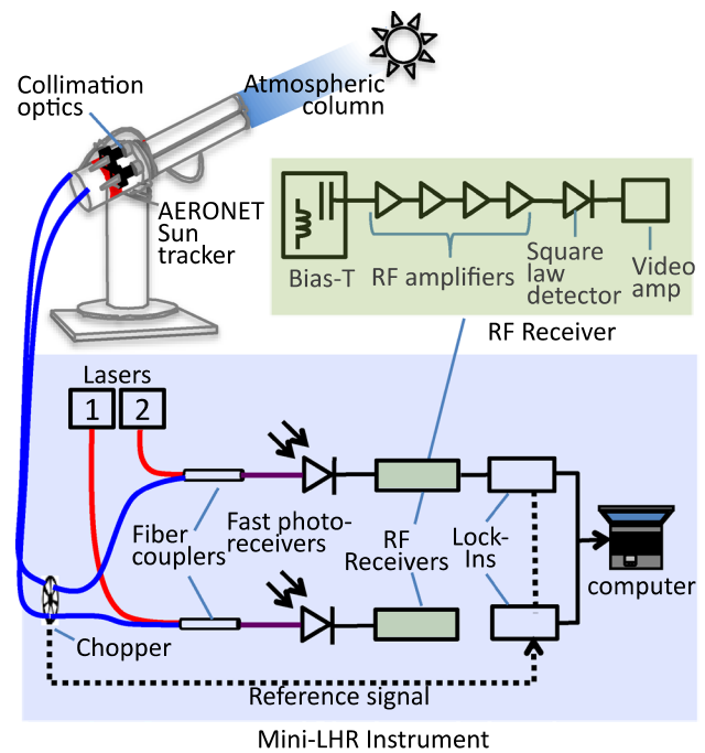
Fig. 1 Mini-LHR instrument schematic (shaded blue) operated in tandem with an AERONET sun tracker (upper left). Sunlight that has passed through CO 2 in the atmosphere is collected with collimation optics and then modulated with an optical chopper. The modulated sunlight is then superimposed with light from a DFB laser (laser 1) at 1611.5 nm in a single-mode fiber coupler, and mixed in a fast photoreceiver (InGaAs detector). A custom RF receiver (shaded green) detects and amplifies the resulting beat signal which is collected with a lock-in amplifier as the laser scans through the CO 2 absorption feature. Components are also shown for a second channel that uses Laser 2 to measure an additional gas such as methane
