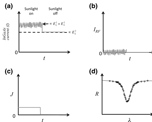
Fig. 2 Pictorial descriptions of the heterodyne process. The interference of sunlight and laser light on the InGaAs detector is shown in (a). The same signal after the DC component has been removed is shown in (b) where I_{\text{RF}} is the RF component of the InGaAs detector current. The output of the RF receiver is depicted in (c) where J (which has a frequency-dependent response to sunlight) indicates the current output from the square-law detector as a function of time. The integrated signal, or irradiance ( R ), is shown in (d) as the laser scans through the wavelengths of the absorption feature
