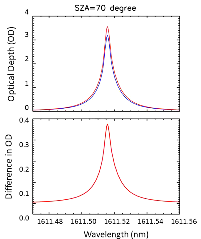
Fig. 5 At large solar zenith angles, the impact of atmospheric refraction is more significant. The top panel shows the modeled total column optical depth for the same line plotted in Fig. 3 for an incident solar zenith angle of 70° at the top of the atmosphere, with atmospheric refraction (in red ) and without ( blue ). The difference in these total column transmittances is shown in the bottom panel where a 10–15% difference in OD is equivalent to 40–50 ppm
