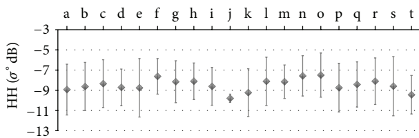
FIGURE 8: Mean and standard deviation of backscatter coefficients on HH.
