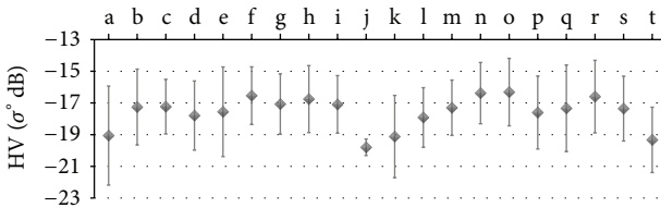
FIGURE 9: Mean and standard deviation of backscatter coefficients on HV.
