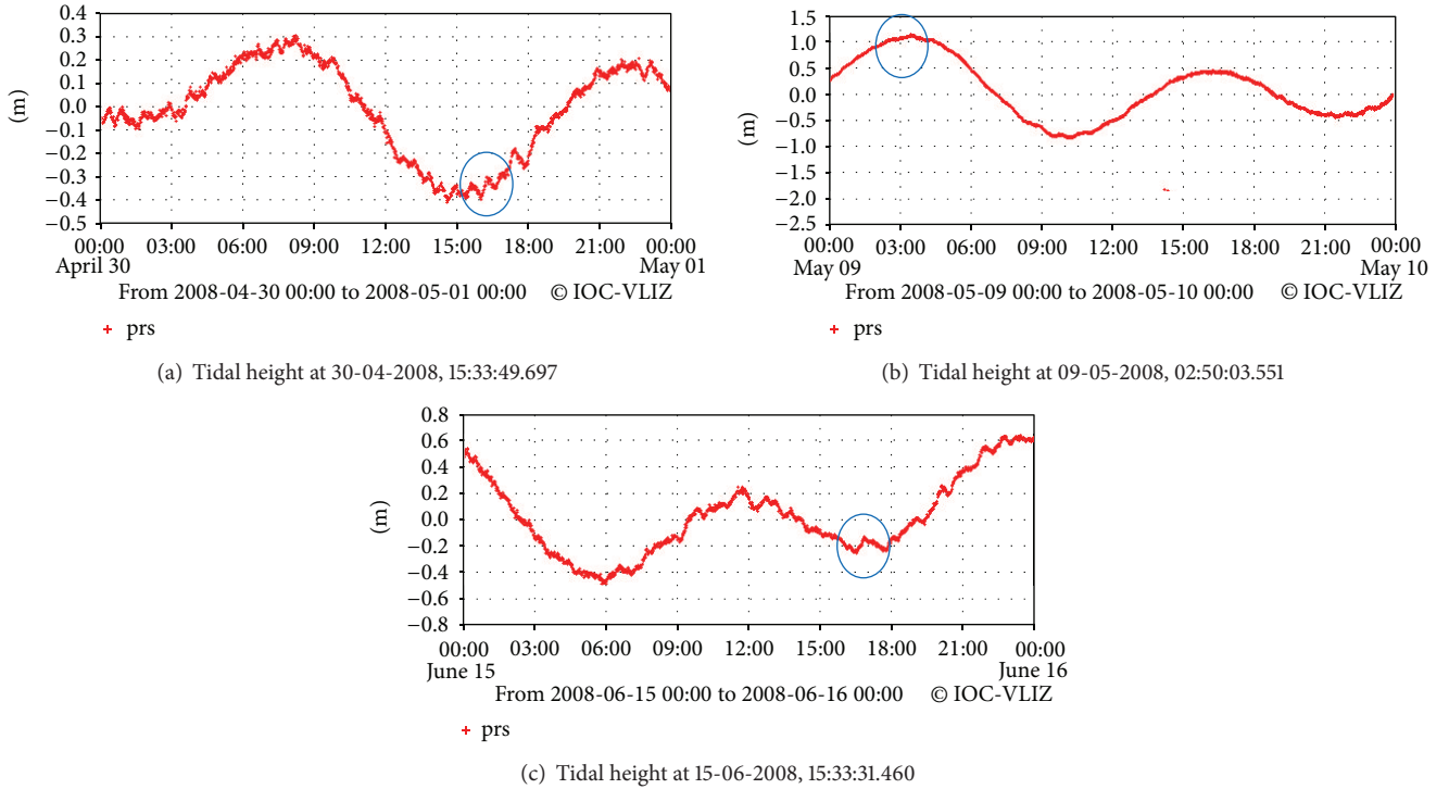
FIGURE 2: Tidal height data corresponding to the same acquisition date with multitemporal ALOS PALSAR polarimetric measurements in Cilacap area (source: http://www.ioc-sealevelmonitoring.org/ ).
