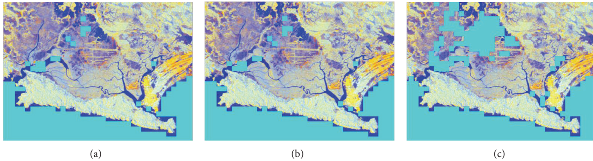
FIGURE 4: Illustration of distribution of flooding and nonflooding at mangrove zone from ALOS PALSAR composite and cyan colors is water (a) tidal height on -0.4 meters, (b) tidal height on -0.2 , and (c) tidal height on 1.0 meter.
