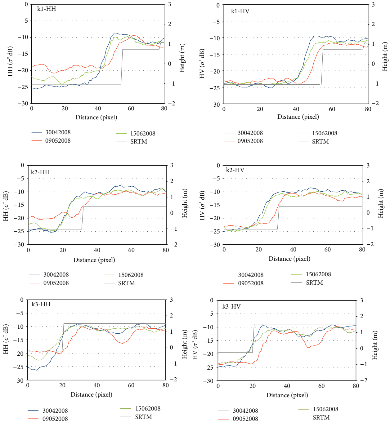
FIGURE 6: Impact of tidal height on ALOS PALSAR polarimetric measurement on HH and HV in Cilacap, Central Java.
