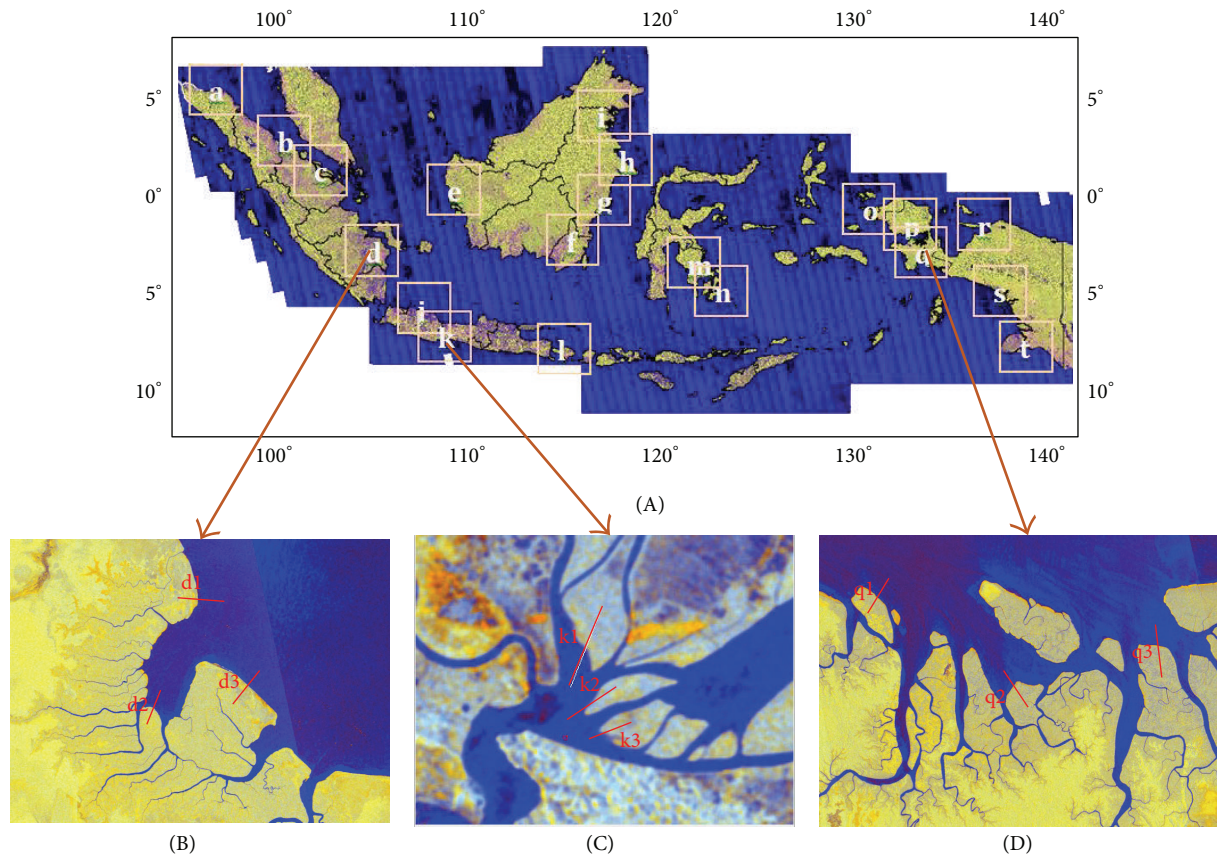
FIGURE 1: Study areas are twenty sites for estimation AGB in Indonesia (A) and ROI in Banyuasin, South Sumatera (B), Cilacap, Central Java (C), and Teluk Bintuni, Papua (D) for investigation impact of topography and tidal height.
