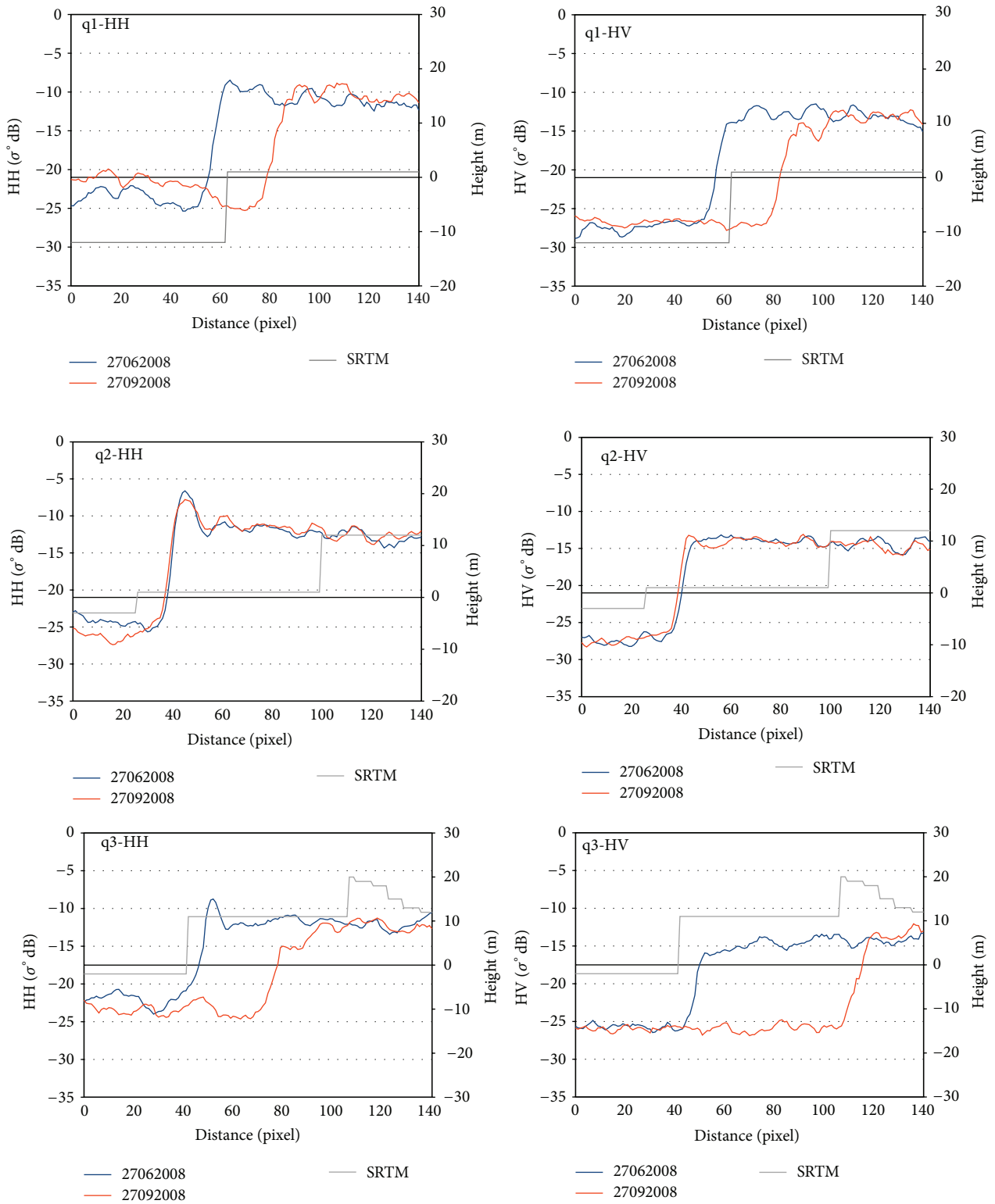
FIGURE 7: Impact of tidal height on ALOS PALSAR polarimetric measurement on HH and HV in Teluk Bintuni, Papua.
