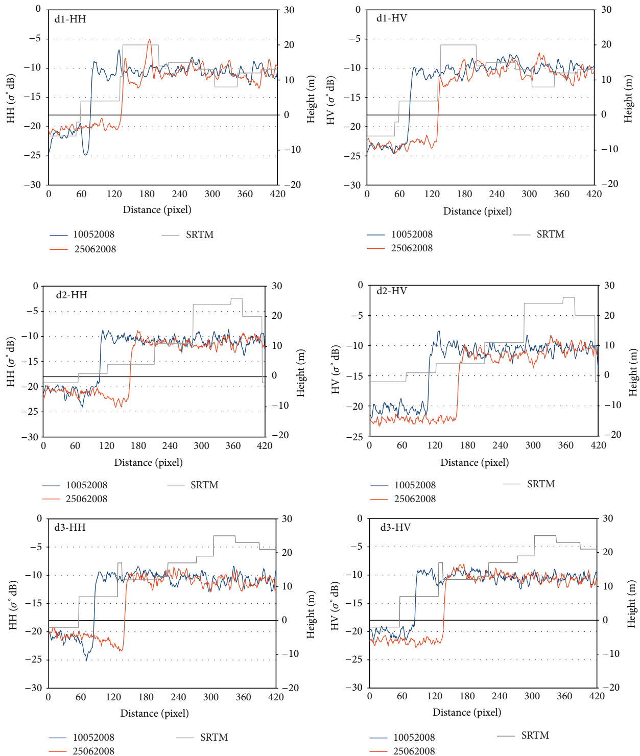
FIGURE 5: Impact of tidal height on ALOS PALSAR polarimetric measurement on HH and HV in Banyuasin, South Sumatera.
