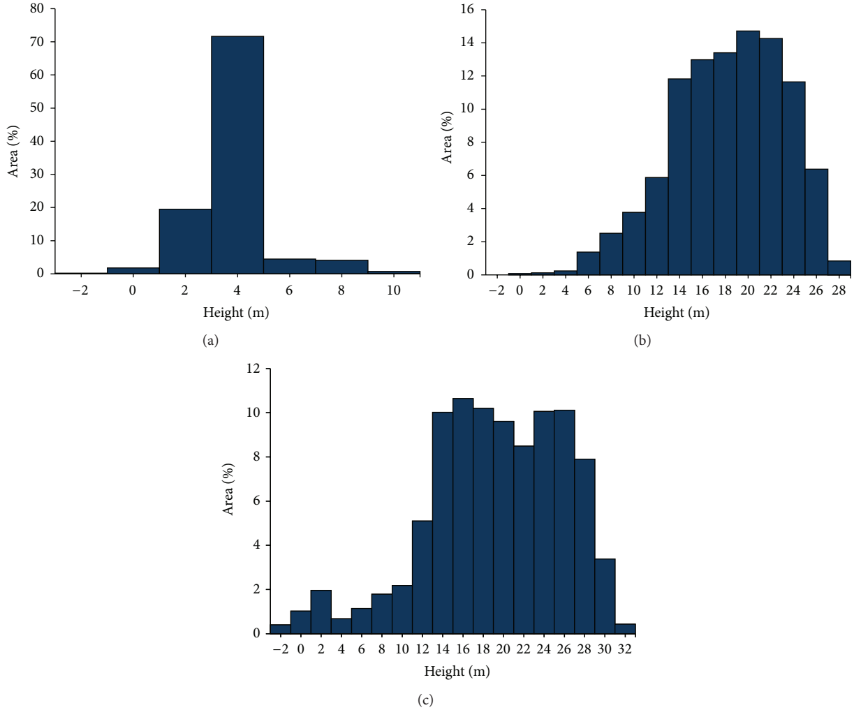
FIGURE 3: Level of topography at study area: (a) Cilacap, West Java, (b) Banyuasin, South Sumatera, and (c) Teluk Bintuni, Papua.
