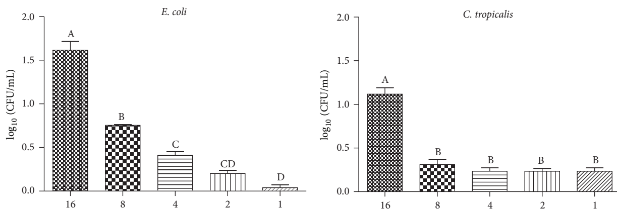
FIGURE 1: Reduction of CFU/mL (log 10 ) number of Escherichia coli and Candida tropicalis biofilm treated with different concentrations of the ethanolic extract of Cochlospermum regium leaves in mg/mL. Different letters represent statistically significant differences found ( p < 0.05 ).
