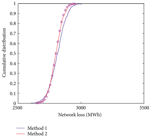
FIGURE 5: Cumulative distribution function of total losses.
