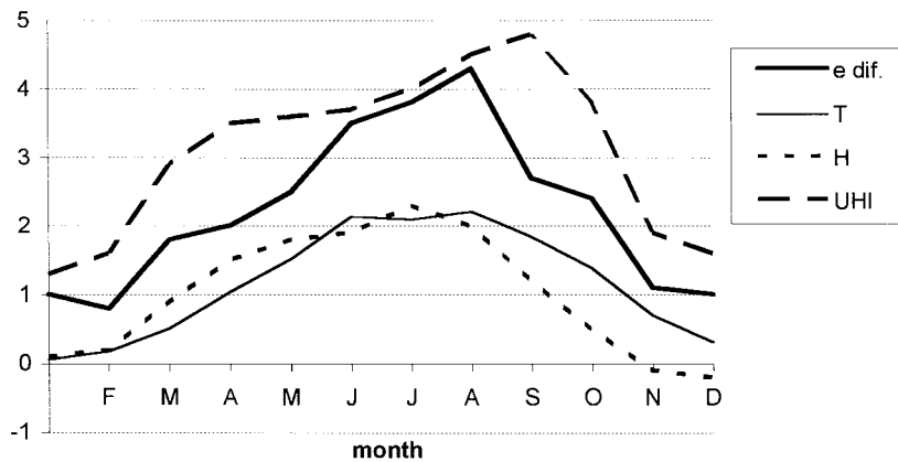
Figure 2. Annual variations of the monthly means of the daily vapour pressure excess of the city ( e —unit 1 hPa), the water temperature of River Tisza ( T —unit 10^{\circ}\text{C} ), the aridity index ( H —unit 1, dimensionless) and the maximum heat island intensity (UHI—unit 1^{\circ}\text{C} ) in Szeged
