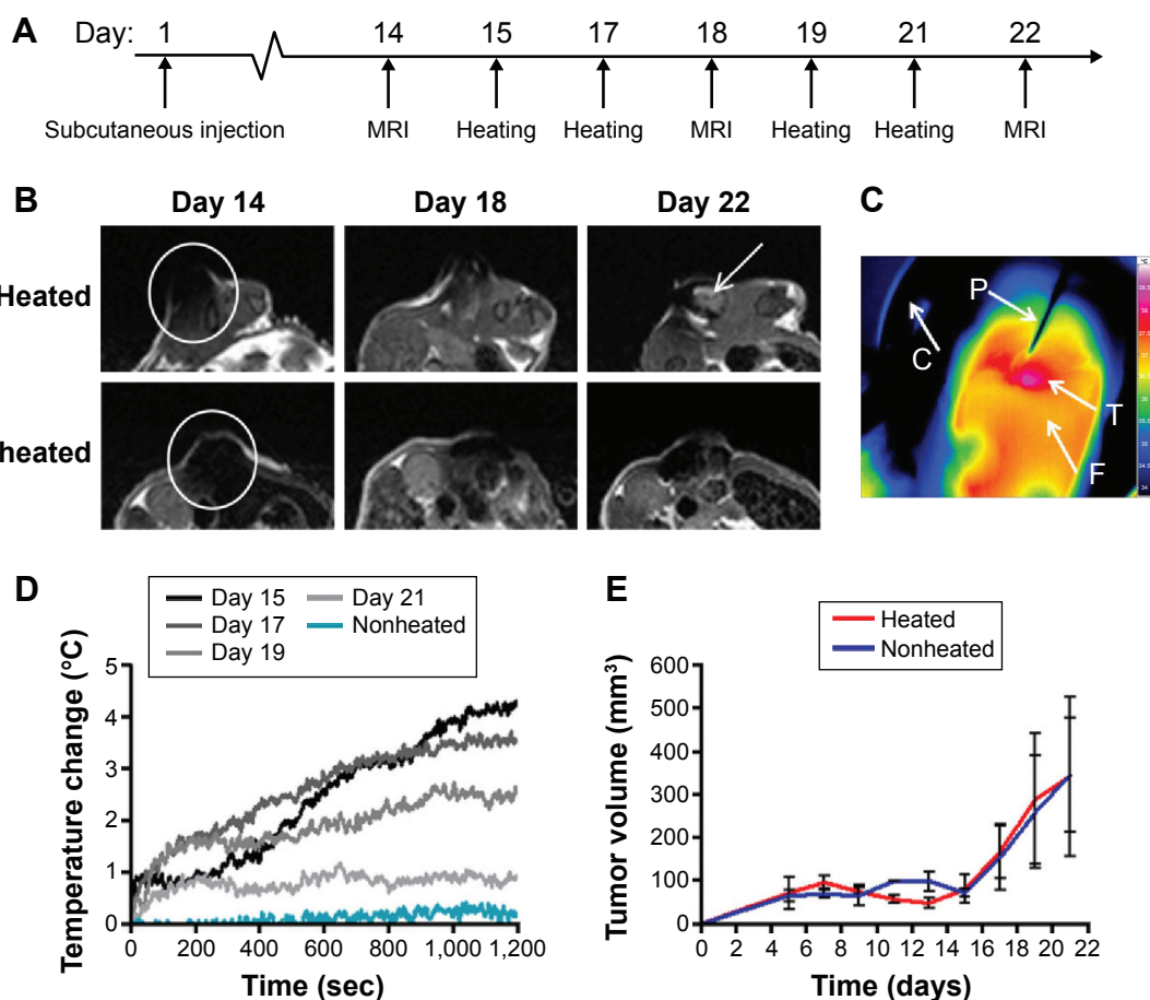
Figure 2 Murine model of OVCAR-3 tumor growth, with and without magnetic heating.
