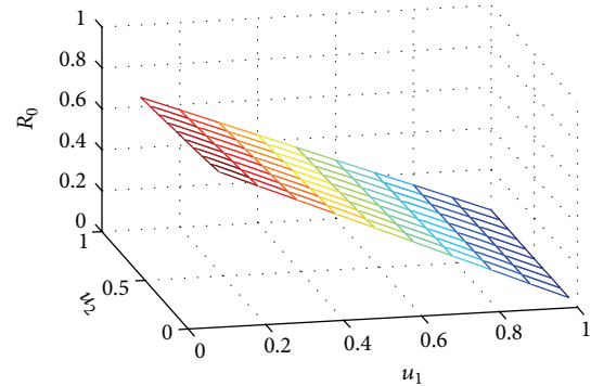
FIGURE 4: The relationship between R_0 and two control variables u_1 and u_2 .
