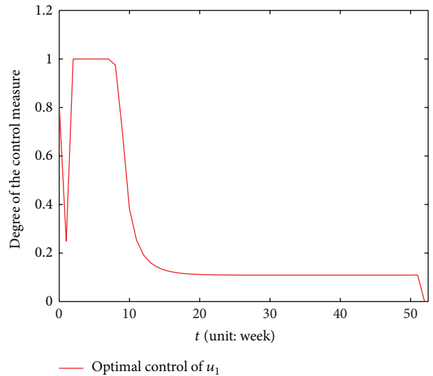
FIGURE 15: Figures of the optimal control u_1 when we choose the weight in objective function are c_1 = 10^4, c_2 = 10^2 .
