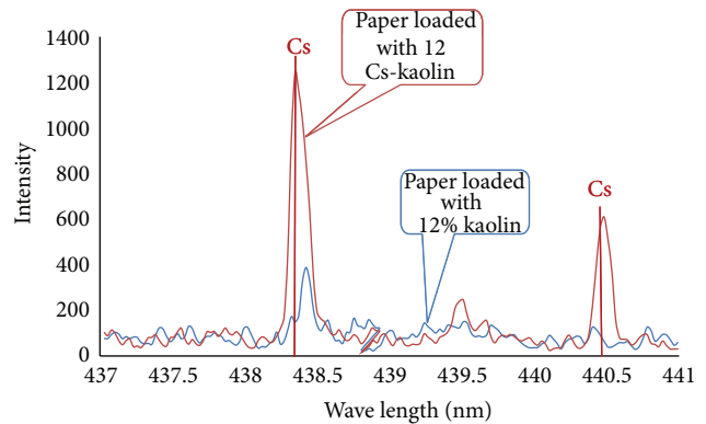
FIGURE 8: LIBS spectra for wood paper hand-sheets loaded by 12% kaolin and 12% Cs-kaolin.
