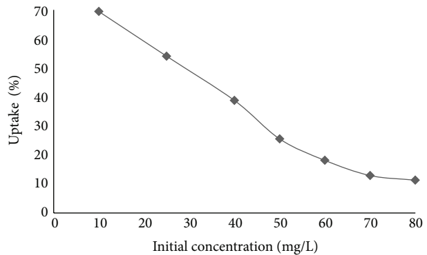
FIGURE 2: Variation of uptake percentage with initial concentration of cesium for its sorption on kaolin. Operating conditions: 50 mL solution, pH = 6, 250 mg kaolin, and shaking time = 40 min.
