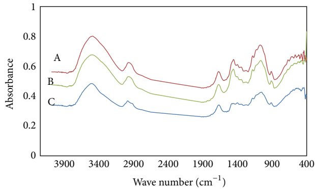
FIGURE 5: FTIR spectra for three \gamma -irradiated wood paper hand-sheets: A: paper loaded with 12% kaolin, B: paper loaded with 12% Cs-kaolin, and C: paper without kaolin.
