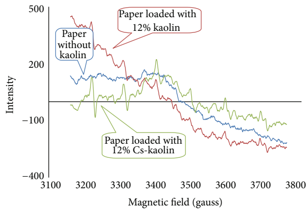
FIGURE 6: ESR spectra for nonirradiated wood paper hand-sheets (without kaolin, 12% kaolin, and 12% Cs-kaolin).
