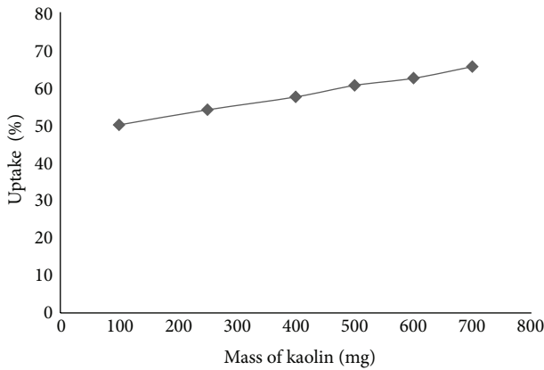
FIGURE 3: Variation of uptake percentage with kaolin mass for cesium sorption on kaolin. Operating conditions: 50 mL solution, [Cs^+] = 25 mg/L, pH = 6, and shaking time = 40 min.
