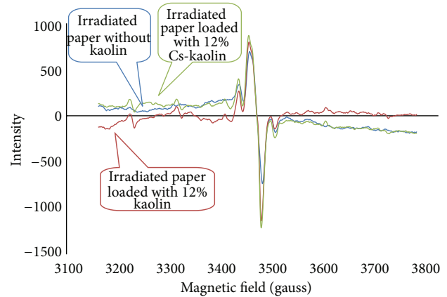
FIGURE 7: ESR spectra for irradiated wood paper hand-sheets (without kaolin, 12% kaolin, and 12% Cs-kaolin).
