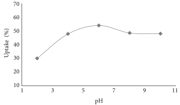
FIGURE 1: Variation of uptake percentage with pH for cesium sorption on kaolin. Operating conditions: 50 mL solution, [Cs^+] = 25 mg/L, 250 mg kaolin, and shaking time = 40 min.
