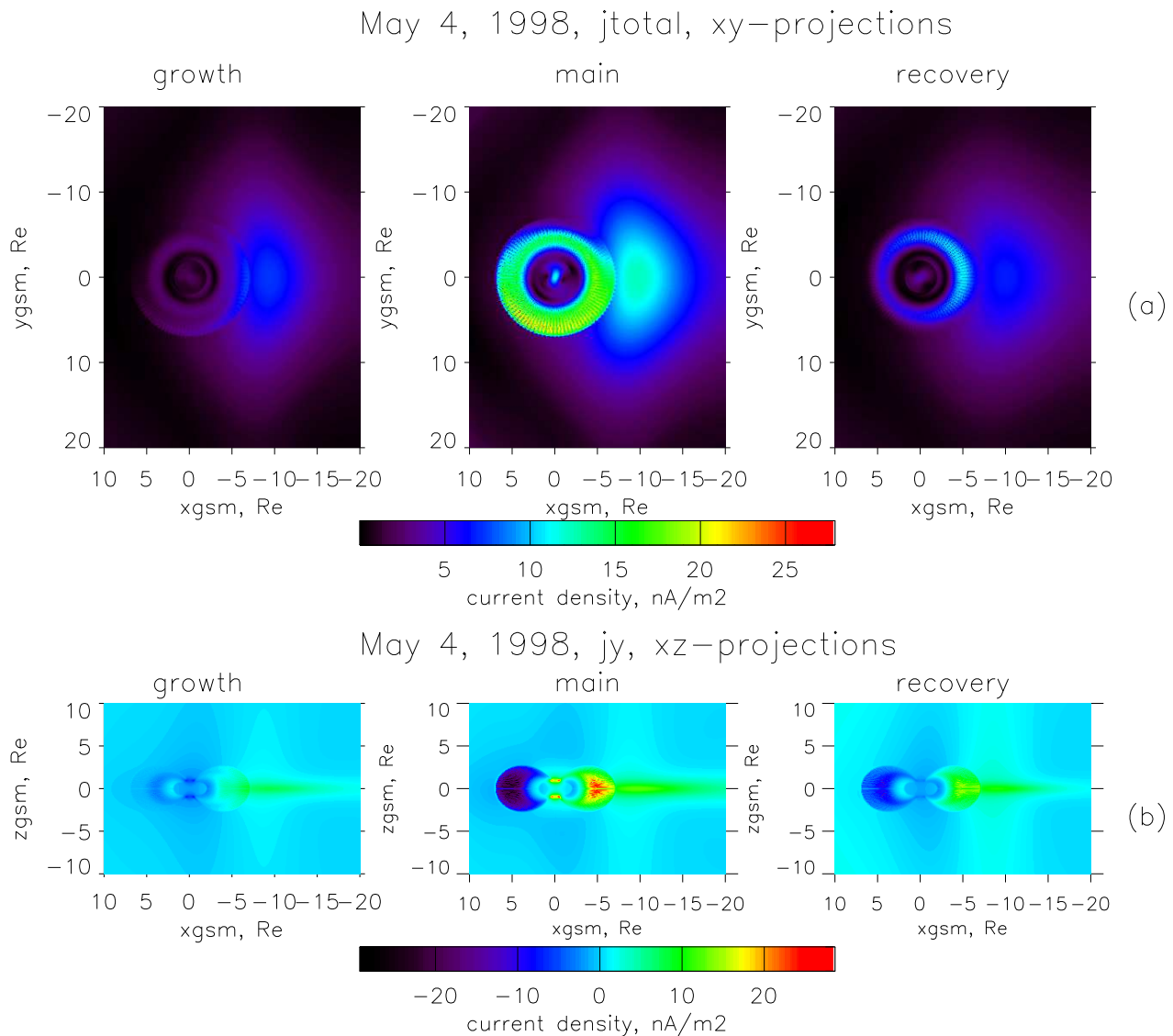
Fig. 12. The model current density in \text{nA/m}^2 in the (a) equatorial and (b) noon-midnight meridian planes for three moments during 4 May 1998 intense storm: (left) before the storm at 01:00 UT, (middle) at the storm main phase at 05:00 UT and (right) during the recovery phase at 10:00 UT.
