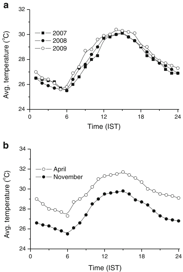
Fig. 4 Annual average diurnal variations of air temperature (°C) observed at Nagercoil for 2007, 2008 and 2009 (a) and average diurnal variations of air temperature in April and November (b). Note that Y-axis scale is different for b
