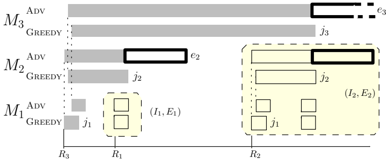
Fig. 1 The instance (I_3, E_3) as applied to GREEDY. The leading jobs of I_3 are gray. Common jobs in GREEDY and ADV schedule are joined using dotted lines. Jobs that only ADV completes are thicker. In this figure, for simplicity we have used one common value \varepsilon_i = \varepsilon ( i = 1, 2, 3 ). We will argue later that this is sufficient for GREEDY
