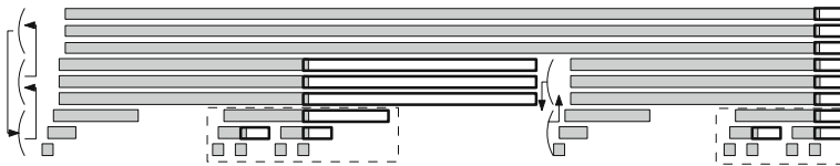
Fig. 2 An instance of (I''_5, E''_5) . The figure shows the schedule of GREEDY, using the same conventions as before. The value of \varepsilon is exaggerated in this figure for clarity; in the actual construction, the first (left most) nine jobs all overlap. On the left and in the middle, groups of three leading jobs are marked, which the adversary schedules on the machines indicated by the arrows. In particular, the last three leading jobs of (I''_5, E''_5) are scheduled later by ADV than by GREEDY, which is why there is no reason to invoke constructions of (I''_1, E''_1) and (I''_2, E''_2) there. In the two instances of (I''_3, E''_3) that are marked by the dotted lines, the schedule of the adversary is as in the previous figure
