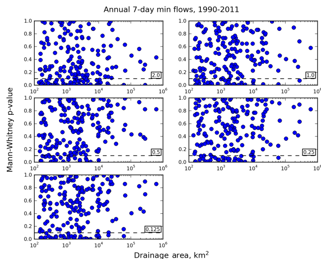
Figure 9. Similar to Fig. 8, but for the 7-day low flows at each streamflow site.
